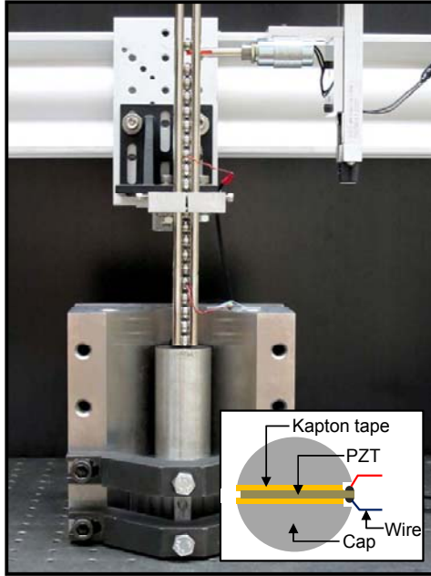
FIG 1. (Color online) Experimental setup consisting of a 20-particle granular chain vertically positioned on the top of a steel cylinder (the linear medium). The inset figure shows the schematic drawing of the instrumented particle, equipped with a piezo-ceramic (PZT) layer.
