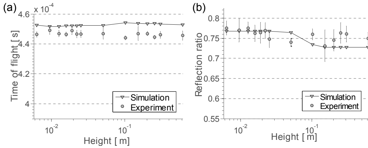
FIG 7. Time of flight and amplitude ratio of the PSWs reflected from the stainless steel slender cylinders as a function of the cylinders' heights. Numerical and experimental data are compared in the magnified Y-axis scale. (a) TOF of the PSW. (b) Amplitude ratio of the PSWs.
