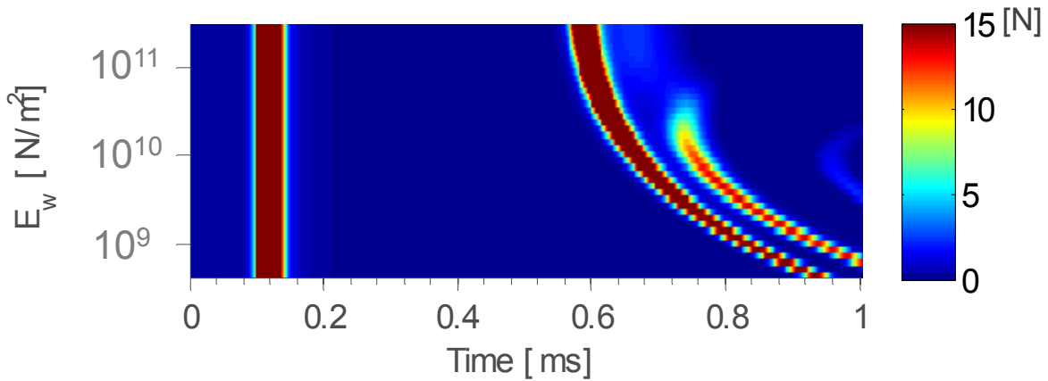
FIG 4. (Color online) Surface plot obtained from numerical simulations showing the formation of primary and secondary solitary waves in the time domain. The Y-axis reports a set of different values of elastic moduli of the linear media adjacent to the chain of spheres. Here, the first vertical line evident at \sim 120 \mu\text{s} from the impact (Time = 0) represents the arrival of the incoming solitary wave. The generation of a reflected SSW is noticeable after a critical value of elastic modulus of the contact. These simulation results are based on the force profile obtained from our numerical model for the particle number 7, and the color bar on the right denotes the amplitude of the force profiles in newtons.
