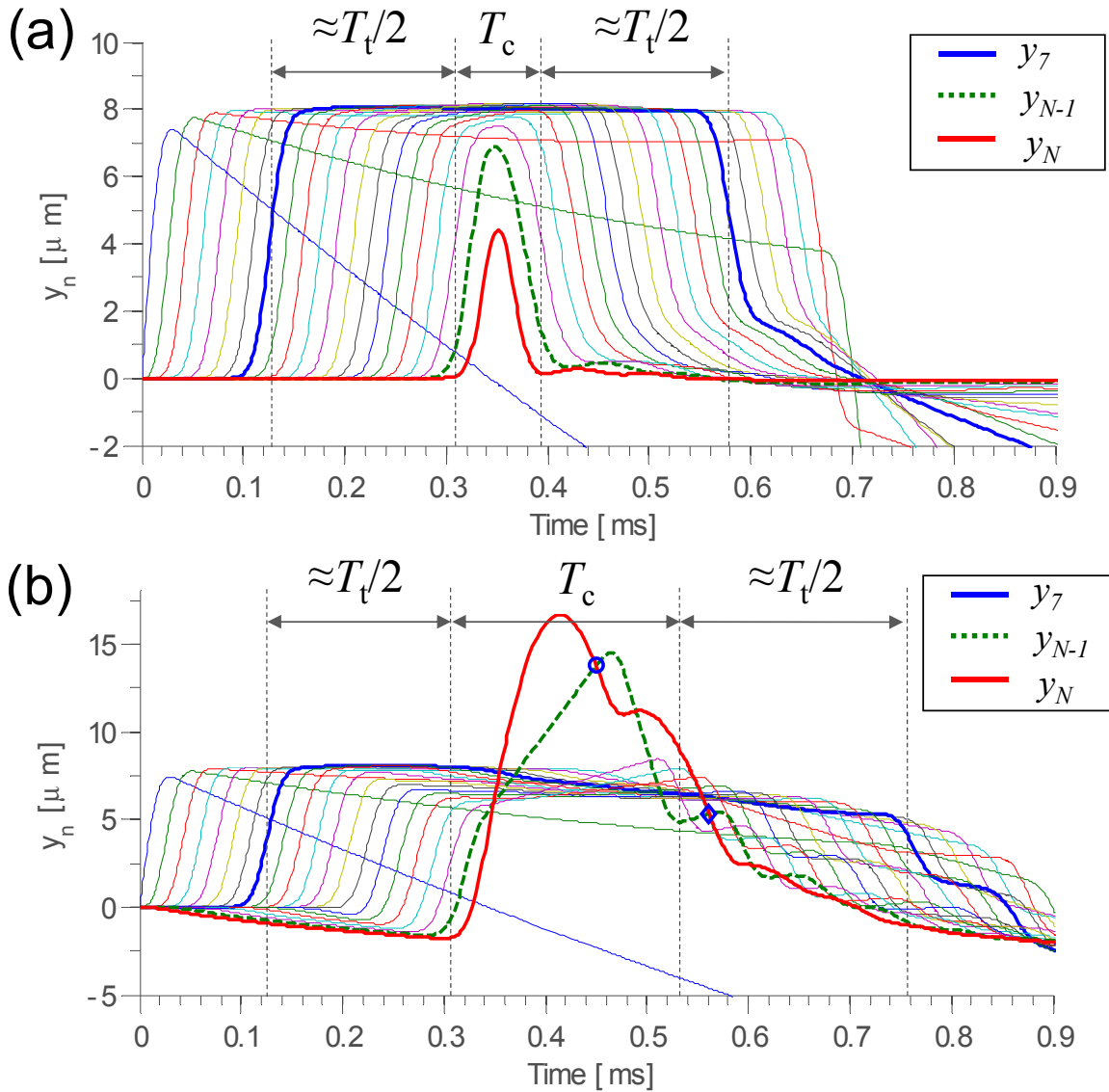
FIG 5. (Color online) Numerical results showing the displacement profiles of the striker bead (first curve on the left) and of the 20 particles composing the chain. (a) The stainless steel wall induces small displacement (4.39 \mu\text{m} ) and short contact time (85 \mu\text{s} ) of the last bead against the bounding wall (bold red line). (b) the PTFE wall allows a larger displacement of the last bead (16.66 \mu\text{m} ) and as a result, a longer contact time (241 \mu\text{s} ) spent on rebounding. Multiple impacts between the last and its neighboring beads are observed in the PTFE case; The first and second collisions occur at 450- \mu\text{s} and 561- \mu\text{s} points as marked in circle and square, respectively.
