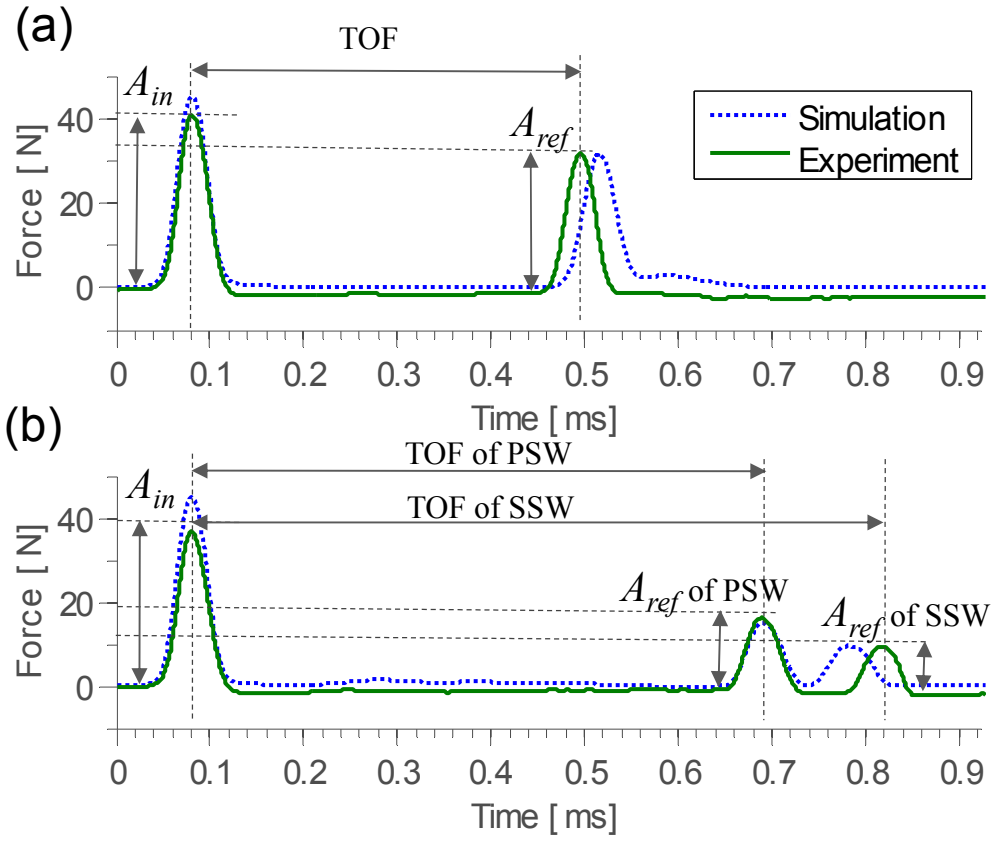
FIG 3. (Color online) Solitary wave propagation measured from the 7th bead in the chain against (a) stainless steel wall and (b) PTFE wall. The time of flight ( TOF ) represents the delay time between the arrival of the incident and the reflected waves. The amplitude ratio ( A_{ref}/A_{in} ) denotes the relative magnitude of reflected solitary waves with respect to the incident solitary waves.
