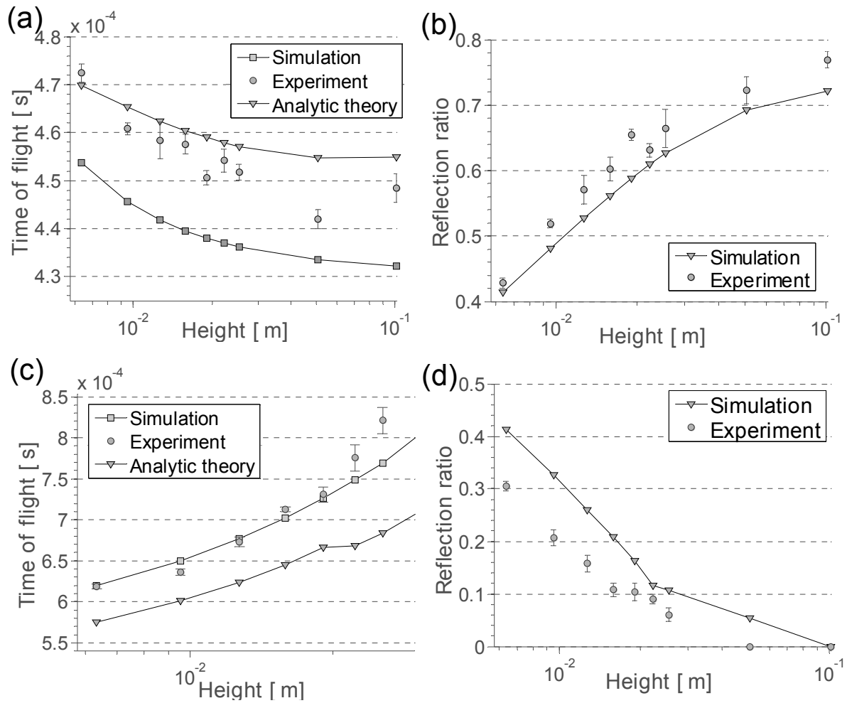
FIG 8. Comparison of experimental, theoretical, and numerical data for the time of flight and amplitude ratio of primary and secondary solitary waves, as a function of the upper layer thickness ( L_u ) in the composite media. (a) TOF for the PSWs. (b) Amplitude ratio for the PSWs. (c) Time of flight for the SSWs. (d) Amplitude ratio of the SSWs.
