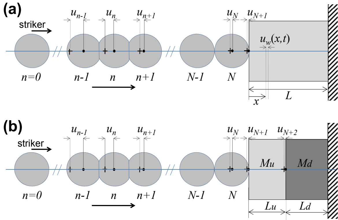
FIG 2. Schematic diagram showing the 1D chain of spherical elements in contact with (a) a uniform linear medium and (b) a composite linear medium.
