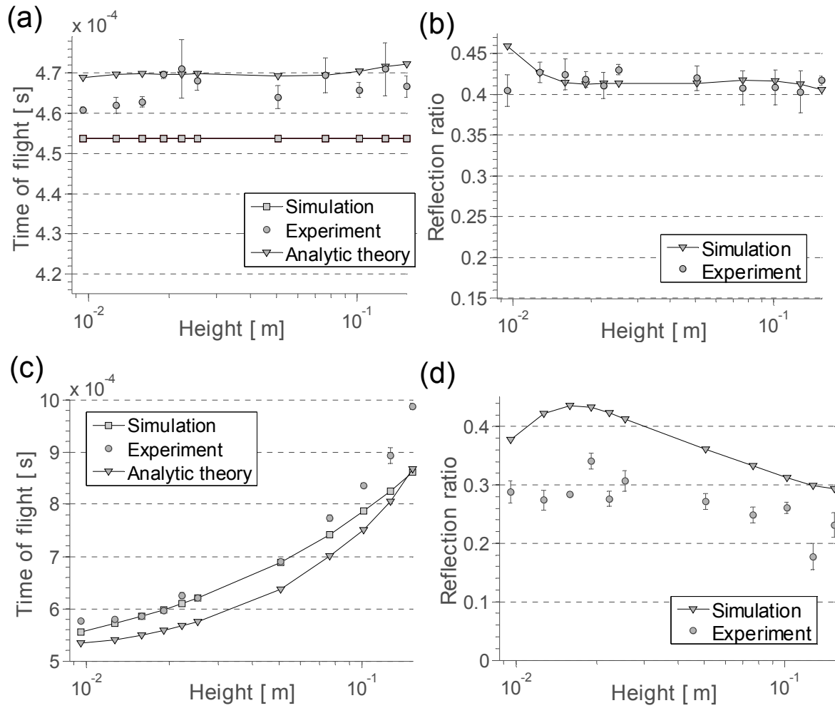
FIG 9. Time of flight and reflection ratio of the primary and secondary reflected solitary waves after the incoming solitary wave interacts with a composite medium with variable lower layer thickness. Numerical and experimental results are represented as a function of lower medium height ( L_d ). (a) TOF of the primary solitary waves. (b) Amplitude ratios of the PSWs. (c) Time of flight of the SSWs. (d) Amplitude ratios of the SSWs.
