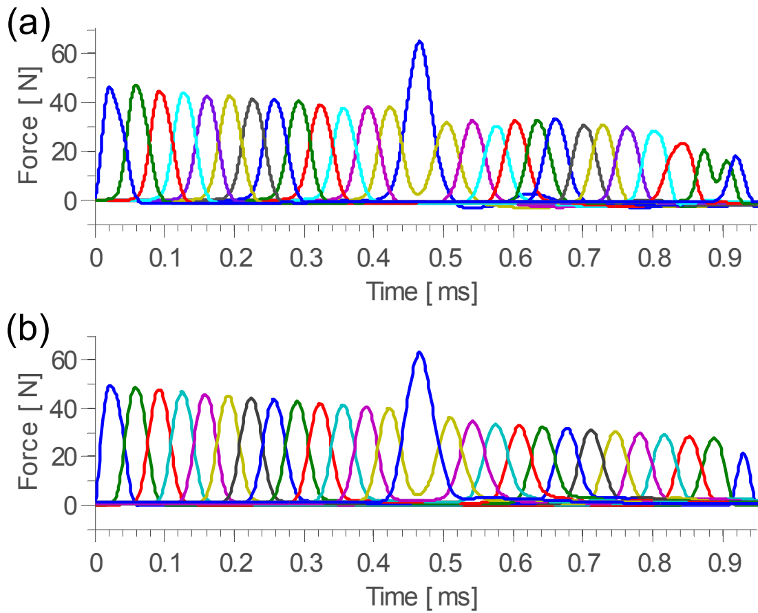
FIG 10. (Color online) Comparison of experimental and numerical force profiles of solitary waves, collected from the particles at the even-numbered positions. The spike in the center is the force measurement from the end-particle. The force profiles prior to this spike represent the solitary wave propagation before the wall reflection, whereas the latter profiles correspond to the reflected solitary waves from the stainless steel bounding wall. (a) Experimental force profiles. (b) Numerical force profiles.
