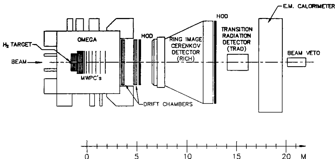
Figure 1: Schematic layout of the experiment
