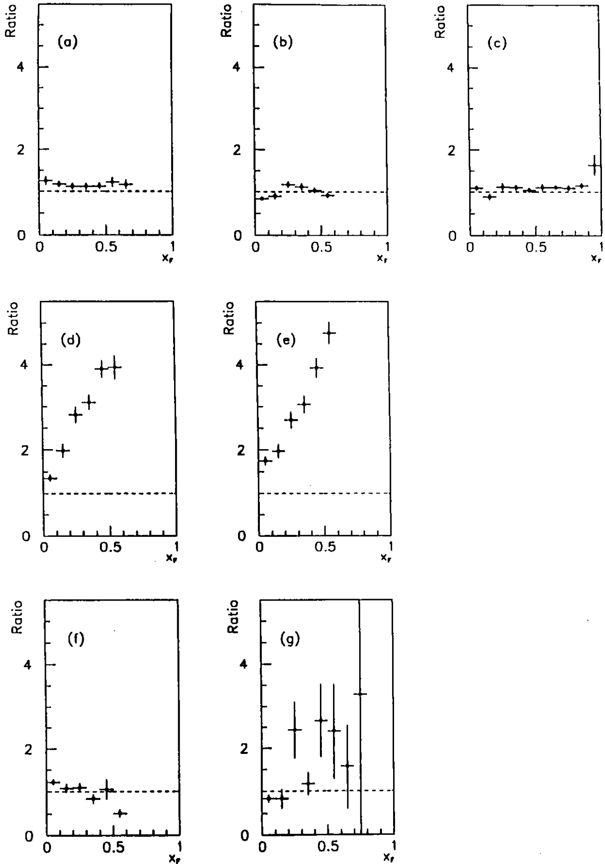
Figure 9: Ratios of cross sections for (a) \sigma(\gamma \rightarrow K^{*0})/\sigma(\gamma \rightarrow \bar{K}^{*0}) (b) \sigma(\pi^- \rightarrow K^{*0})/\sigma(\pi^+ \rightarrow \bar{K}^{*0}) (c) \sigma(K^+ \rightarrow K^{*0})/\sigma(K^- \rightarrow \bar{K}^{*0}) (d) \sigma(K^- \rightarrow \bar{K}^{*0})/\sigma(\pi^+ \rightarrow \bar{K}^{*0}) (e) \sigma(K^+ \rightarrow K^{*0})/\sigma(\pi^- \rightarrow K^{*0}) (f) \sigma(\pi^+ \rightarrow K^{*0})/\sigma(\pi^- \rightarrow \bar{K}^{*0}) (g) \sigma(K^- \rightarrow K^{*0})/\sigma(K^+ \rightarrow \bar{K}^{*0}) . The ratios are shown as functions of x_F . The invariant cross sections are consistent between low and high energies and so ratios of averages are shown.
