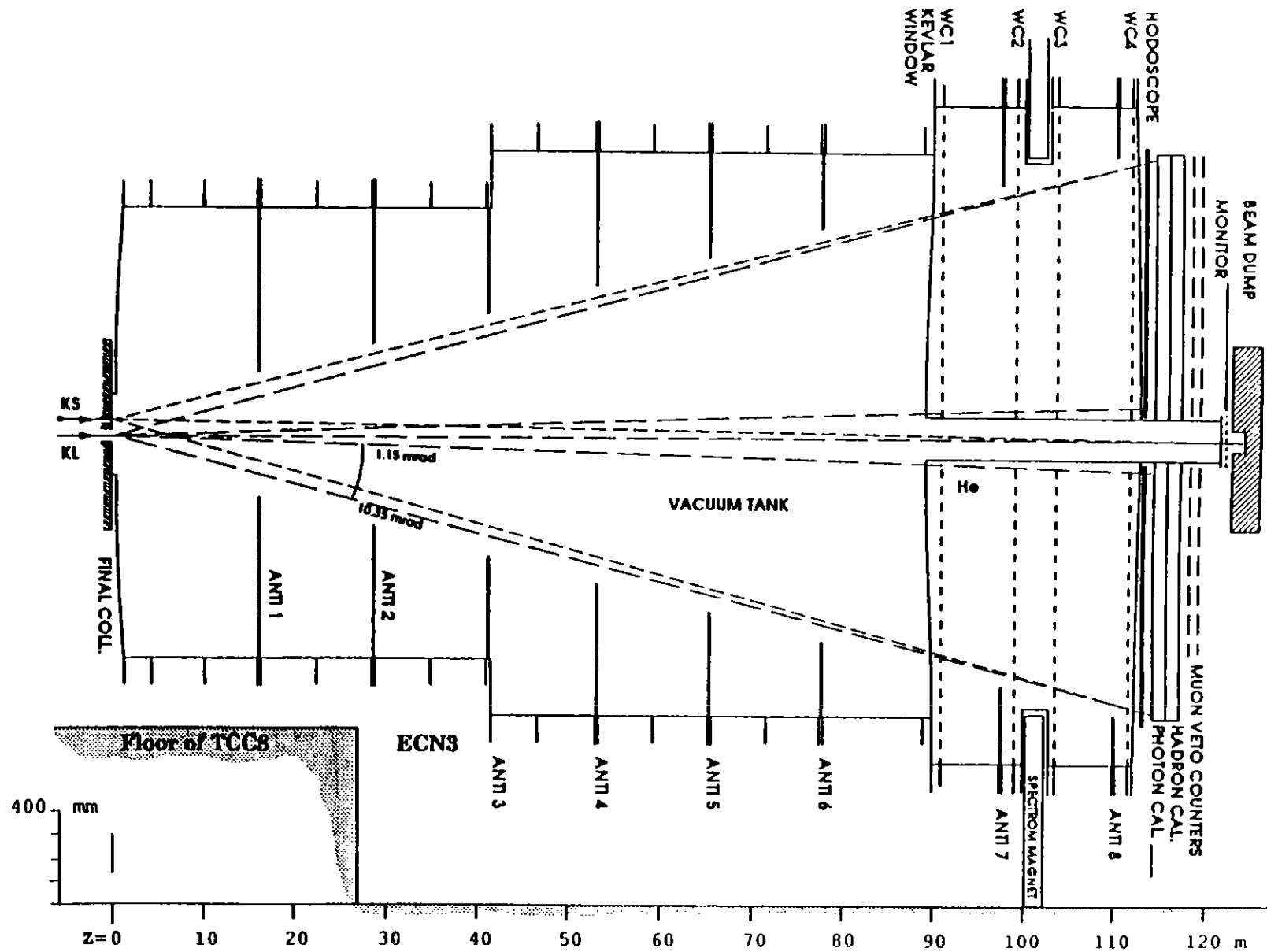
Fig. 1 Schematic layout of the NA48 experiment: the vacuum tank and the magnetic spectrometer are shown.
