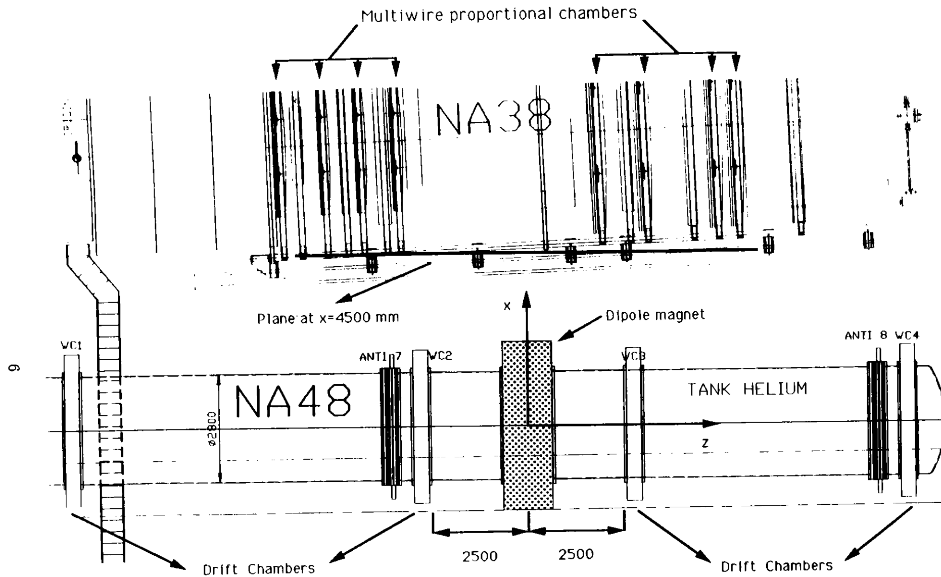
Fig. 2 Layout of the NA48 magnetic spectrometer in the North Area ( dimensions in mm - scale 1:100 ).
