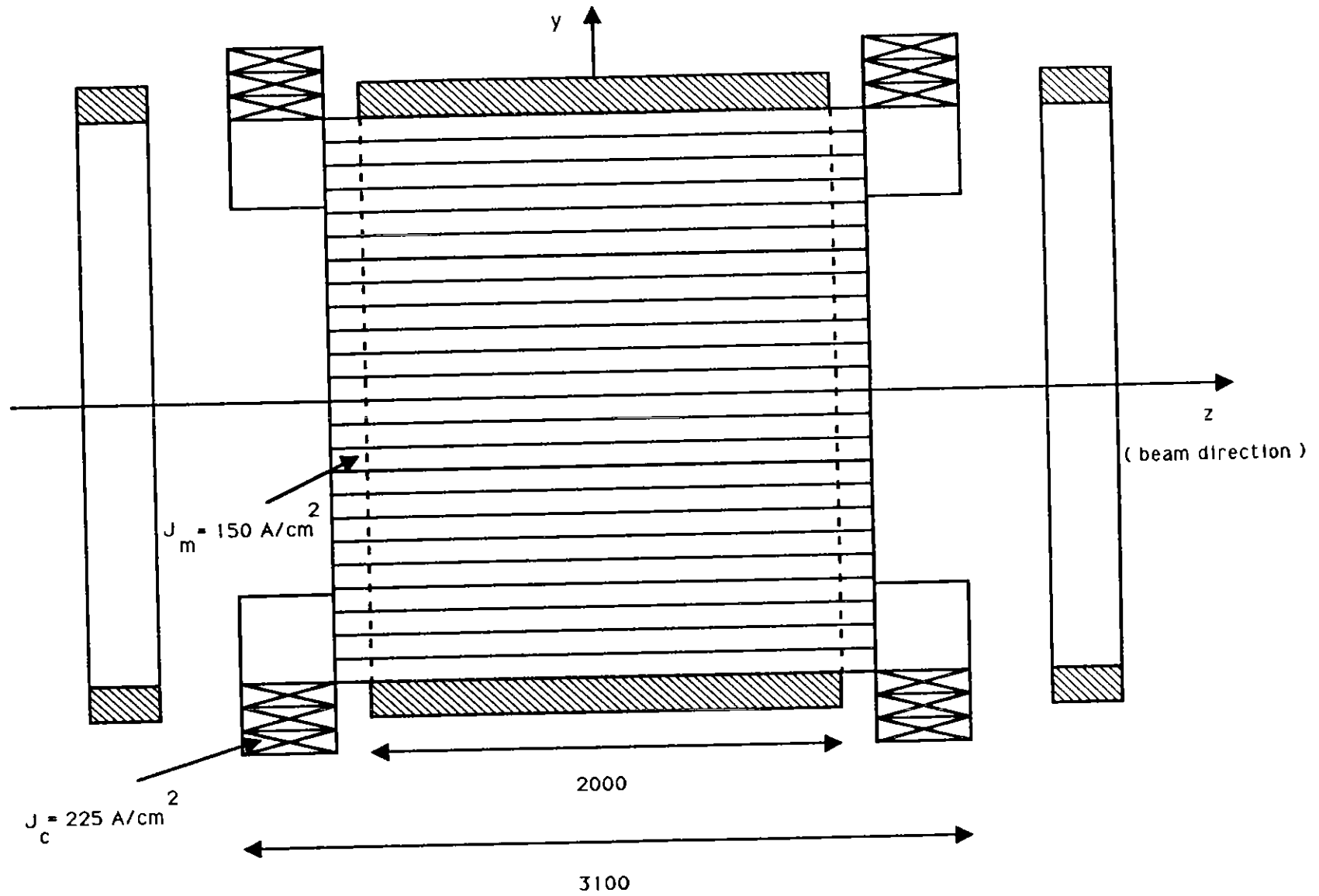
Fig. 3b Magnet section in the symmetry plane x = 0 containing the beam direction ( dimensions in mm - scale 1:25 ).
