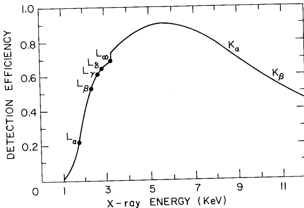
Fig. 15. X-ray detection efficiency with 12 \mu\text{m} mylar.
