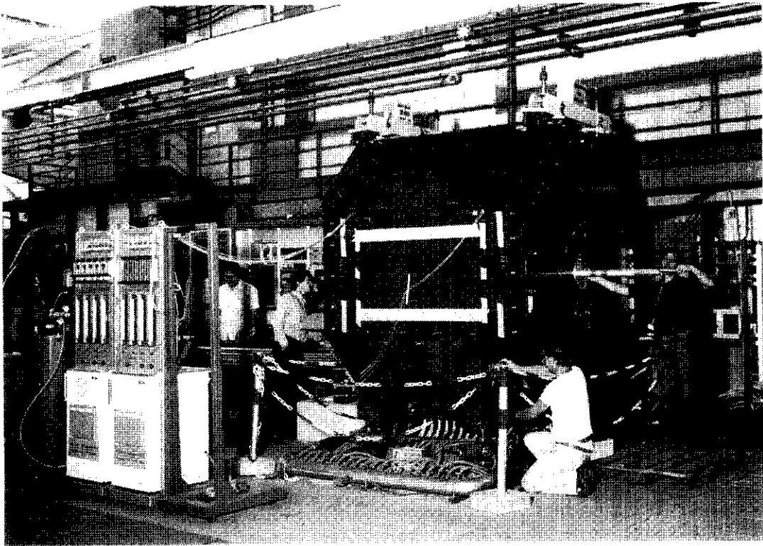
Fig. 2. The ASTERIX version of the DM1 solenoidal spectrometer 3) in the CERN PS South Hall, after shipment from LAL Orsay, during magnetic field measurements in July 1982.
