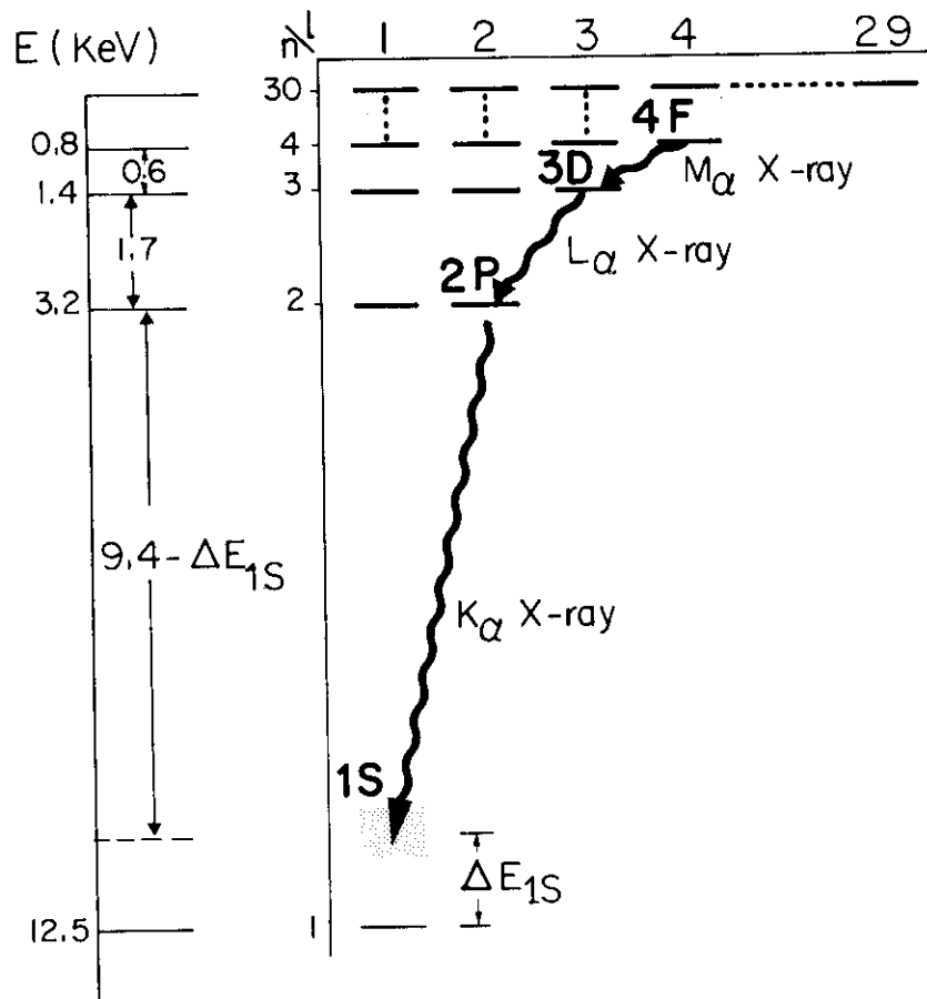
Fig. 3. Levels of the p\bar{p} atom and some detectable X-ray transitions
