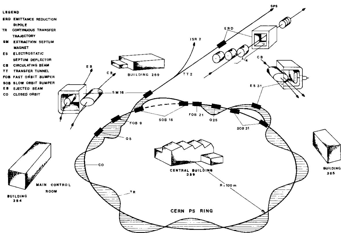
Fig. 1 Synoptic diagram of continuous transfer process
