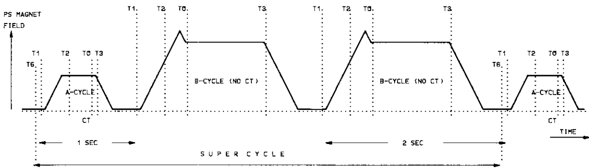
Fig. 6 Timing interrupts for equipment driver synchronization
