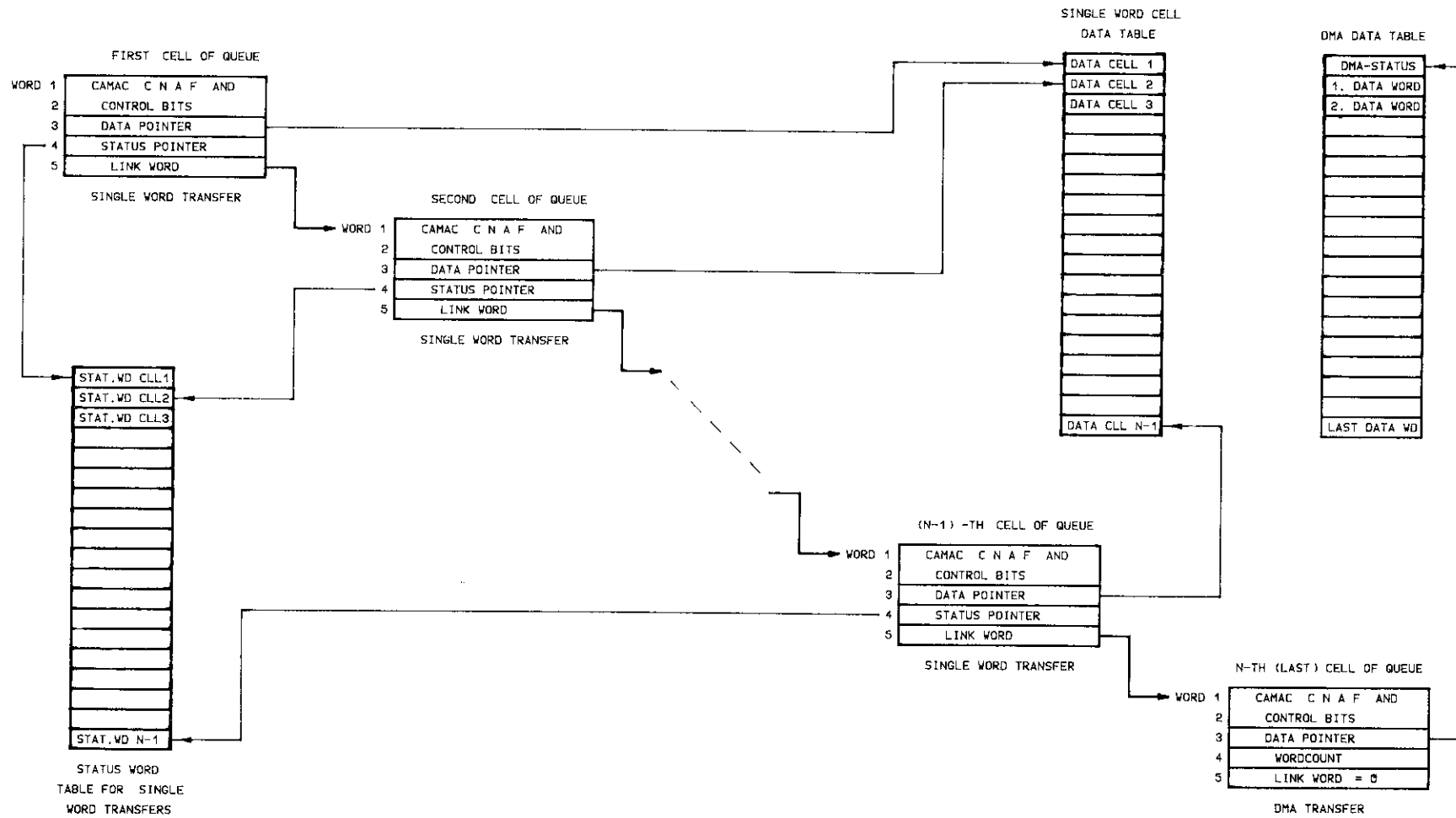
Fig. 4 Cell queue for CAMAC driver input and related data tables
