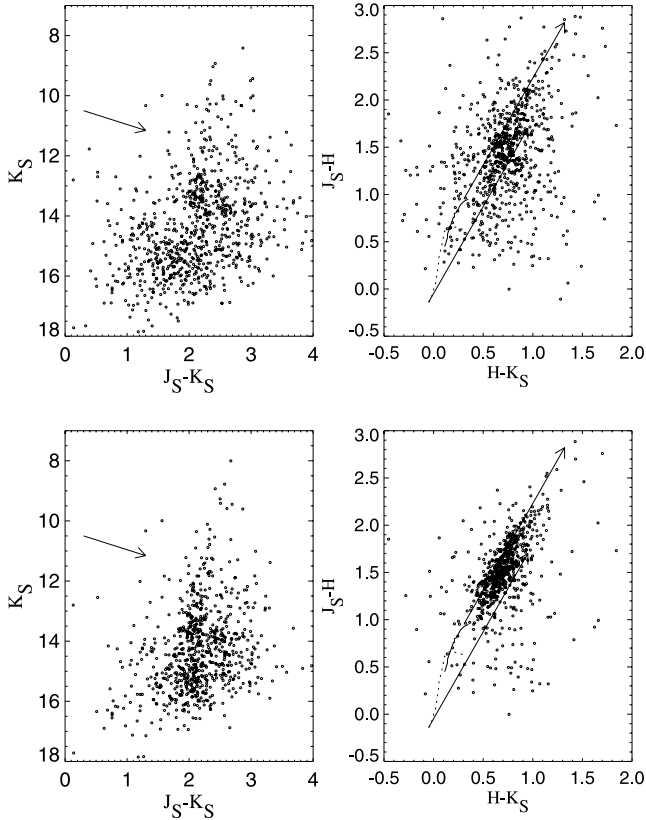
Figure 14. Top: SofI short-exposure observations of Mercer 5. Bottom: the same diagrams, but containing simulated, differentially reddened and distance-shifted data based on observations of NGC 6539 (see text for details).
