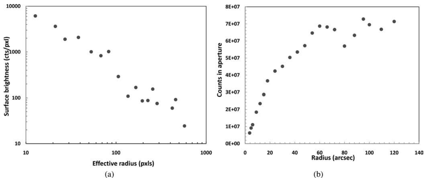
Figure 3. (a) Logarithmic surface brightness profile in mean count pixel -1 (1 pixel \equiv 0.4 arcsec), centred on revised position of cluster. No background has been subtracted in this plot. (b) Total count versus radius, background subtracted with its value set to stabilize differential counts at >1 arcmin (see text).
