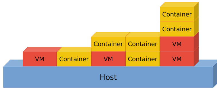
Fig. 1 Examples of different configurations of layers of execution environment
