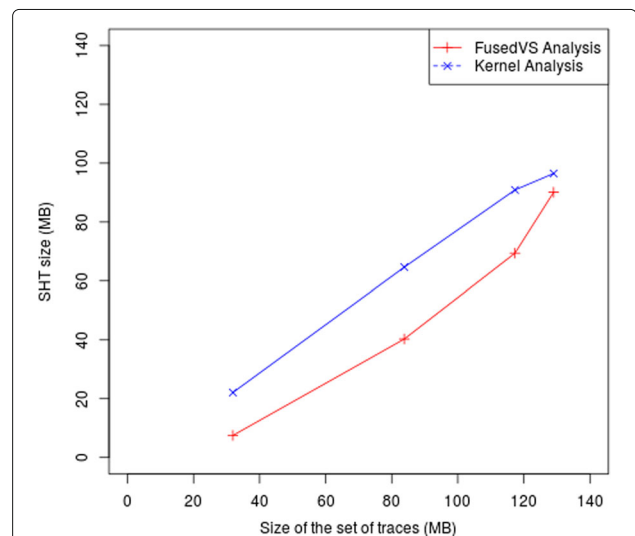
Fig. 20 Comparison of the SHT’s size between FusedVS analysis and Kernel analysis
