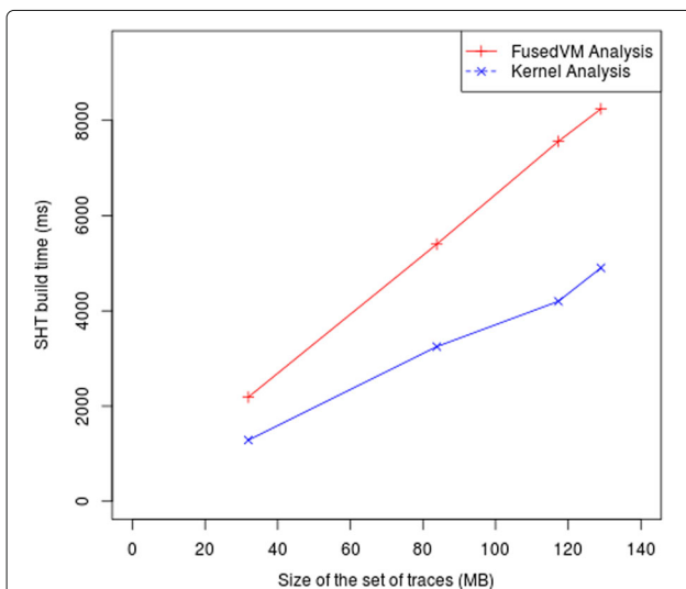
Fig. 19 Comparison of construction time between FusedVS analysis and Kernel analysis
