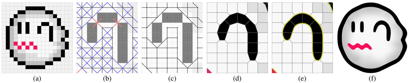
Figure 3: Overview of our algorithm. (a) Input Image (16 × 16 pixels). (b) Initial similarity graph with crossing edges. The blue edges lie inside flat shaded regions, so they can be safely removed. In case of the red lines, removing one or the other changes the result. (c) Crossing edges resolved. (d) Reshaped pixel cells reflecting the connections in the resolved similarity graph. (e) Splines fit to visible edges. (f) Final result with splines optimized to reduce staircasing (Image © Nintendo Co., Ltd.).
