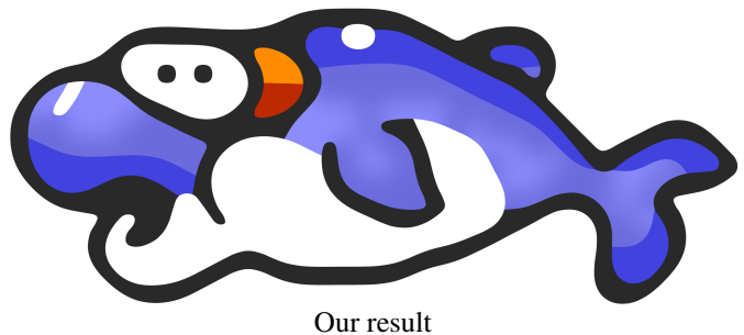
Figure 1: Naïve upsampling of pixel art images leads to unsatisfactory results. Our algorithm extracts a smooth, resolution-independent vector representation from the image, which is suitable for high-resolution display devices. (Input image © Nintendo Co., Ltd.)
