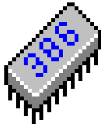
“386” Input (25×31 Pixels)
