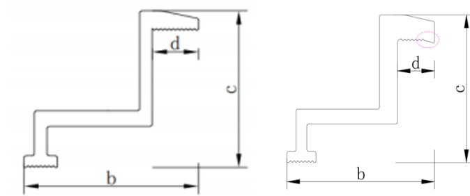
Fig. 5 (a) regular clamp
