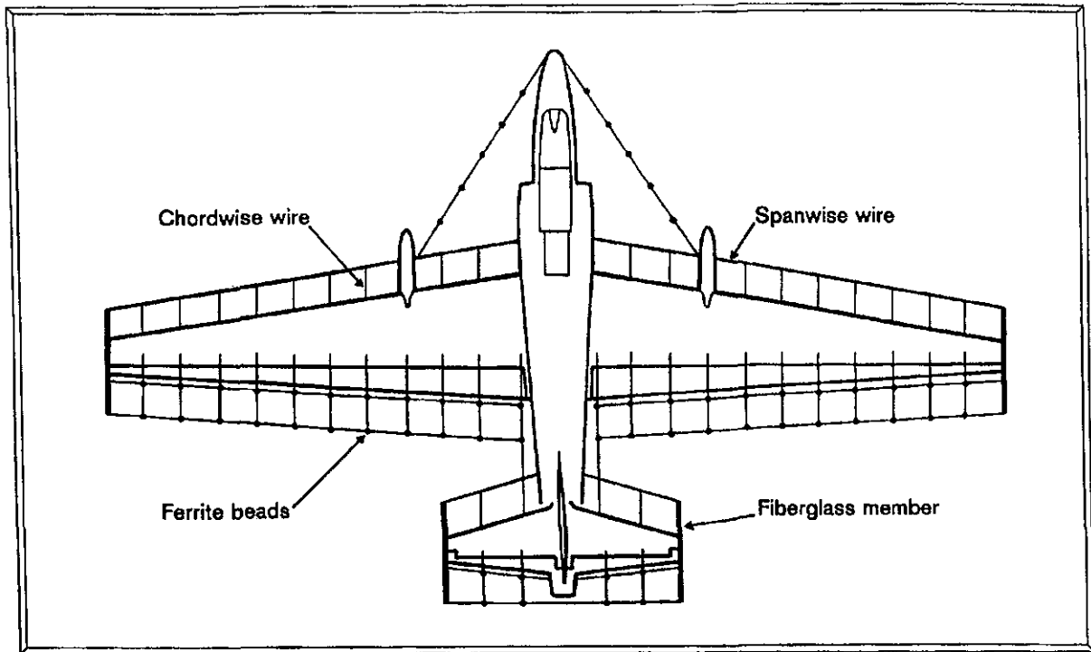
"Trapeze" antiradar attachments to the U-2
