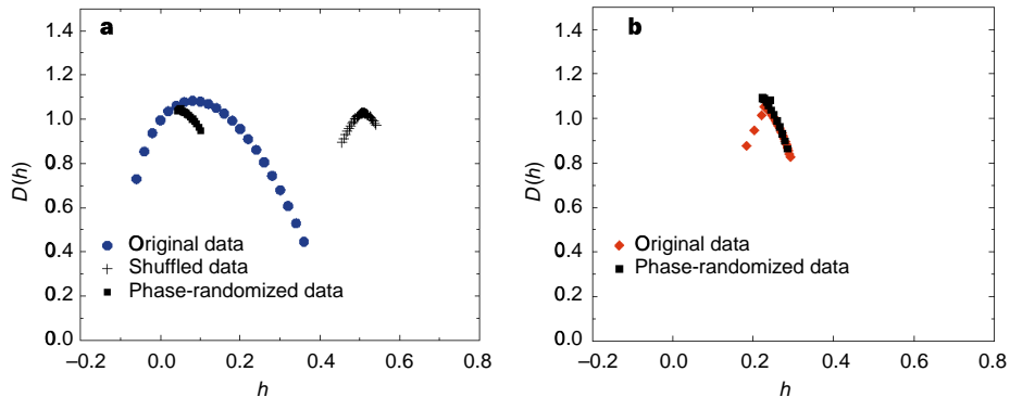
Figure 5 Nonlinearity and Fourier phases. a. The fractal dimensions D(h) for a 6-h daytime record from a healthy subject. After reshuffling and integrating the increments in this interbeat-interval time series, so that all correlations are lost but the distribution is preserved, we obtain monofractal behaviour—a very narrow point-like spectrum centred at h = H = 1/2 . Such behaviour corresponds to a simple random walk. A different test, in which the 1/f scaling of the heartbeat signal is preserved but the Fourier phases are randomized (that is, nonlinearities
