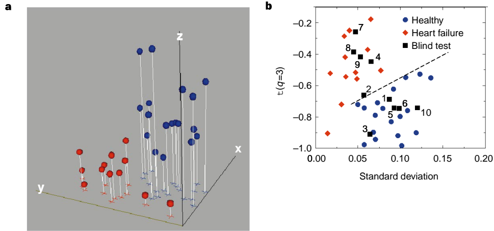
Figure 4 Discrimination method based on the multifractal formalism. a. Each subject's dataset in the database is characterized by three quantities. The first quantity (z-axis) is the degree of multifractality, which is the difference between the maximum and minimum values of local Hurst exponent h for each individual. The degree of multifractality is zero for a monofractal. The second quantity (y-axis) is the exponent value \tau(q = 3) characterizing the scaling of the third moment, Z_3(a) . The third quantity (x-axis) is the standard deviation of the interbeat intervals. Blue spheres, healthy subjects; red spheres; heart-failure subjects. This multifractal approach discriminates healthy from heart-failure subjects. b. Discrimination method based on multifractal formalism for the 'blind' datasets. The y-axis is the exponent value \tau(q = 3) , and the x-axis is the standard deviation of the time series of interbeat intervals. Black squares show the results for the datasets of the blind test. Two of the heart-failure subjects (closest to the origin) do not fit as clearly in either group; however, they are clearly identified as unhealthy in a because their degree of multifractality (z-axis) is close to zero (these two subjects are indicated by the red spheres in a that are closest to the origin). These cases demonstrate that a single exponent is not sufficient to describe the complexity of a heartbeat time series.
