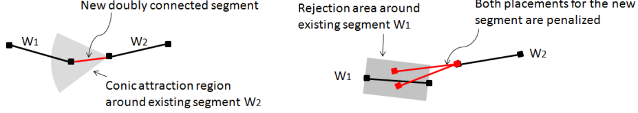
Fig. 2. (a)Attraction interaction creates doubly connected segment (b) Rejection interaction
