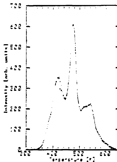
Figure 2 TLD-100 glow curve obtained after \alpha -irradiation.
