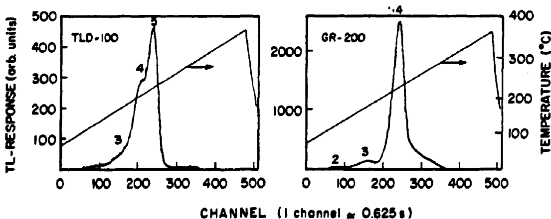
Fig.1 Glow curves of TLD-100 (10 mGy ^{60}Co gamma rays) and GR-200 (1 mGy ^{60}Co gamma rays) read out under the same procedure ( 1 °C s^{-1} ). Note the difference in scale of the TL response and the difference in dose.
