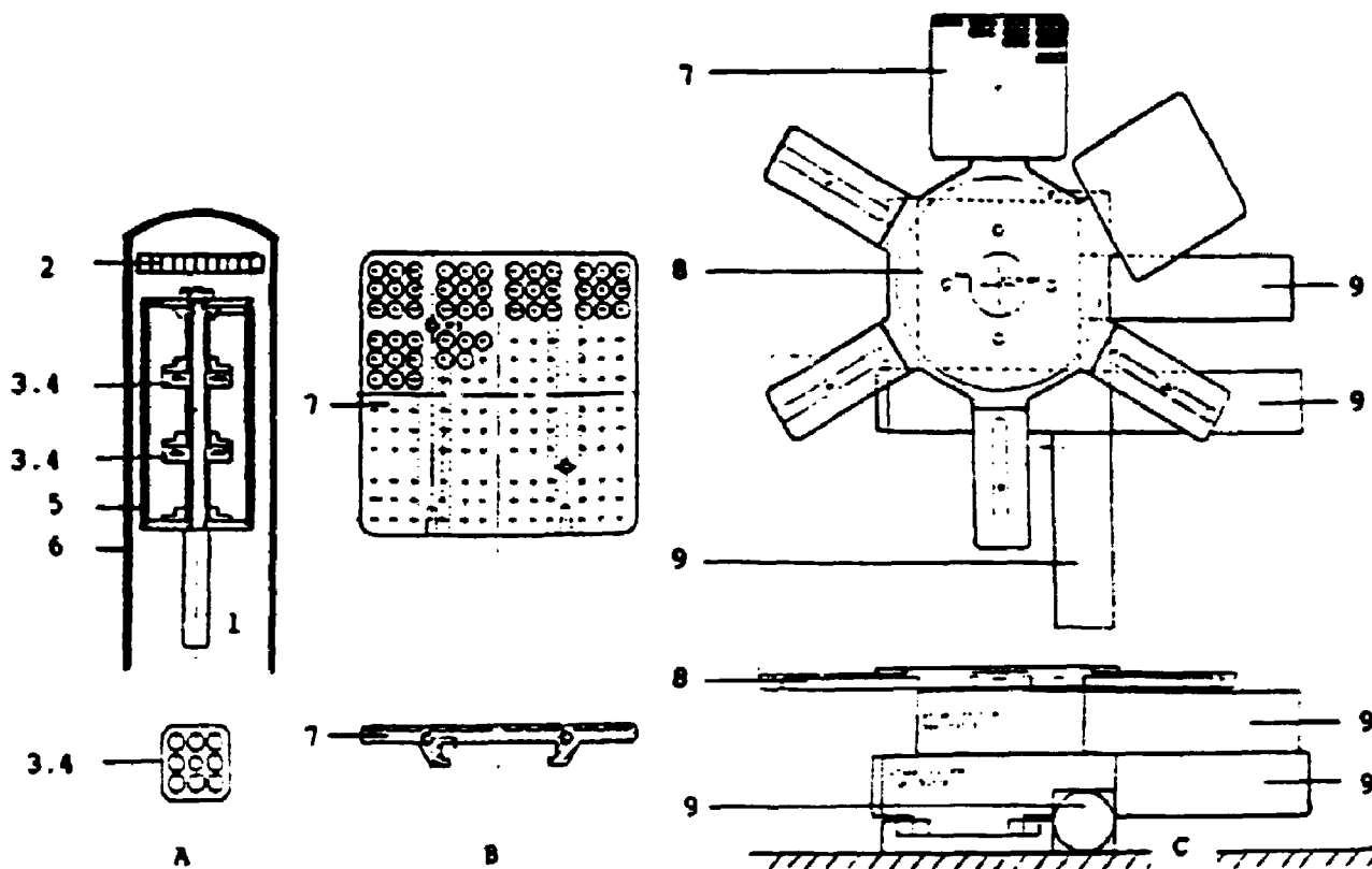
Fig. 2. A The TLD-holder. The calamity TLDs (2) are positioned at the top. Below them are the environmental TLDs (3), which are placed in nylon (4) and surrounded by two-millimetre copper (5). Both TLD-groups are embedded in PVC (6). B The pick-out platforms. The TLDs are placed on these platforms when they have to be annealed or read out. C The readout table (8). The pick-out platforms are placed on the "legs" of the table, so that the TLDs can be accurately positioned under the TLD-reader by stepping motors (9).
