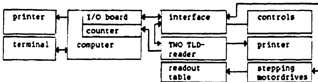
Fig. 3. Simplified blockdiagram of the electronics.
