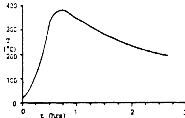
Fig.4. TLD annealing temperature curve
