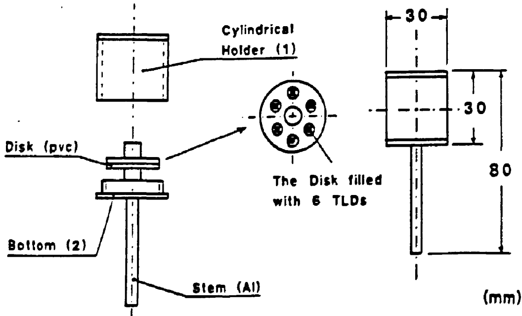
Fig. 1: Dosimeter applied for environmental monitoring at RIVM with a 2.5 mm copper cylindrical holder to provide for energy compensation. In case of \text{LiF:Mg,Ti} part 1 and 2 consist of PVC.
