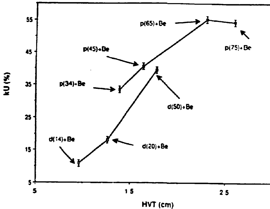
Fig. 2 : Variation of the k_U value of TLD700 as a function of the HVT (at a depth of 2cm and a 10cm x 10cm field size).
