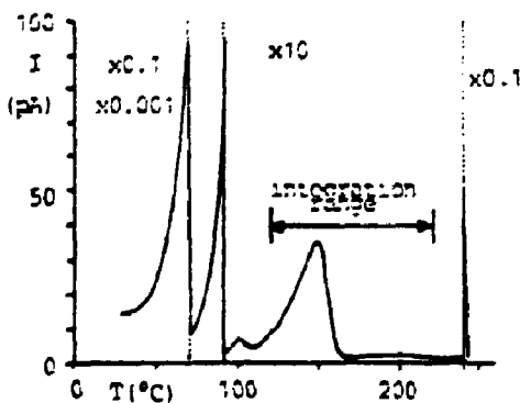
Fig.3. TLD 100 Glow curve and integrating range
