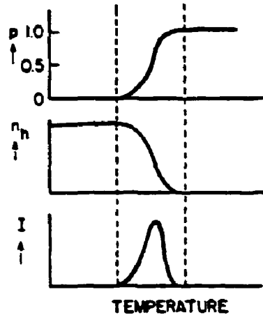
Fig. 2 Relationship between probability p to escape from a trap, the number of trapped holes n_h at the recombination centres and the thermoluminescence intensity I(t) .
