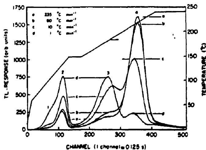
Fig. 4 Change in glow curve pattern of GR-200 for different cooling rates in the annealing procedure starting at 240 °C for 10 min. Glow curves originate of the same chip irradiated to the same dose level (1 mGy).
