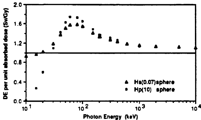
Fig. 1. Dose equivalents at 0.07 and 10 mm depths on the principal axis of the ICRU sphere per unit absorbed dose to air in free air for photons incident in a plane parallel beam 4 .
