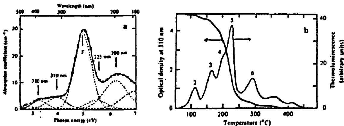
Fig. 6 a. Absorption spectrum for irradiated TLD-100. Dashed lines: calculated Gaussian absorption bands. b. Thermoluminescence and annealing of the 310 nm absorption band in TLD-100 irradiated to 10^3 Gy (Adopted from McKeever 7 )
