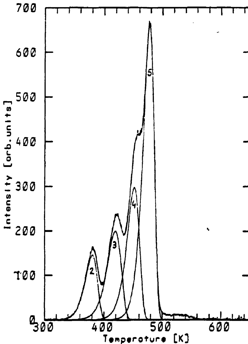
Fig.4 Glow curve of TLD-100 after a pre-irradiation annealing of 1 h 400 °C and fast cooling and irradiation with ^{60}\text{Co} gamma rays. The measured glow curve is fitted with four first order peaks with a fitting procedure described elsewhere 3 .
