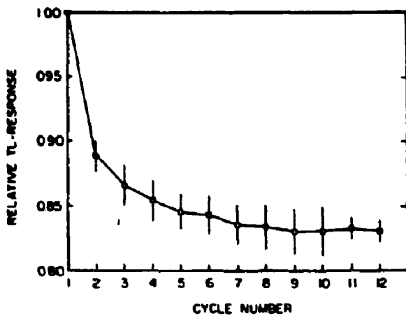
Fig.3 Change in sensitivity of GR-200 after repeated use. Every cycle involves annealing (10 min at 240 °C followed by a fast cooling i.e. 235 °C min -1 ), irradiation (1 mGy 60 Co gamma rays) and standard readout. Every point is the average ± standard deviation of 15 chips.
