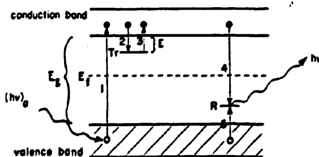
Fig 1. Simple two-level model for thermoluminescence. Allowed transitions: (1) ionization through absorption of radiant energy; (2) en (5) trapping; (3) thermal release; (4) radiative recombination and the emission of light.
