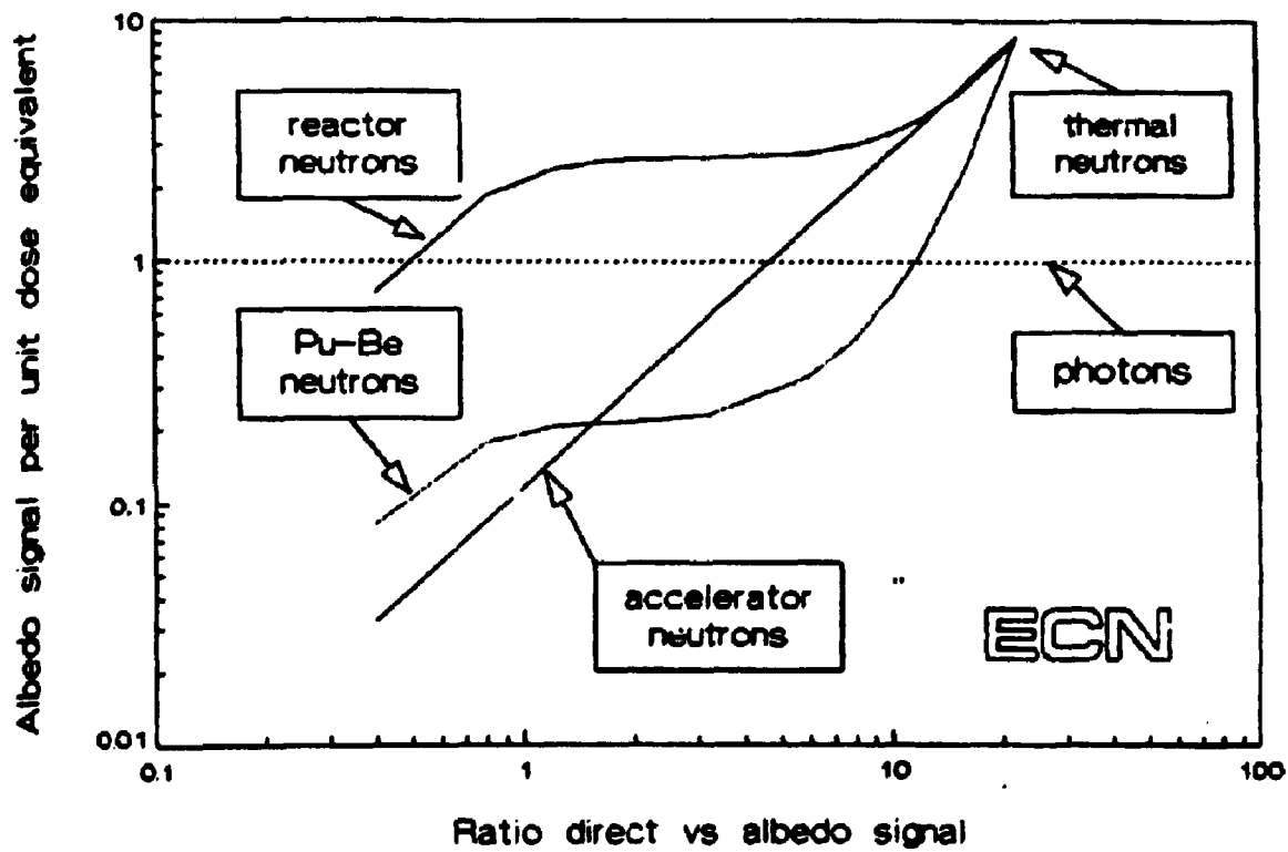
Figure 2. Neutron response to different sources
