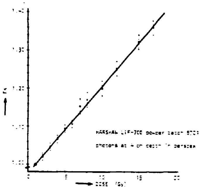
Fig. 3. The ratio F_s (eq.3) plotted versus dose. Supralinearity is already obvious at the radiotherapy dose level.
