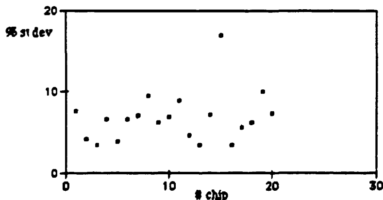
Fig. 1. Standard deviations of 20 lithiumborate chips - 5 readings.
