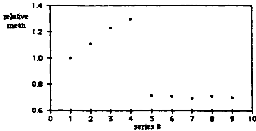
Fig. 2. Relative mean of read-out of 20 LiF chips irradiated with 2.16 Gy. Irradiation 1-4 was after annealing at 300°C, irradiations 5-9 after annealing at 400°C.
