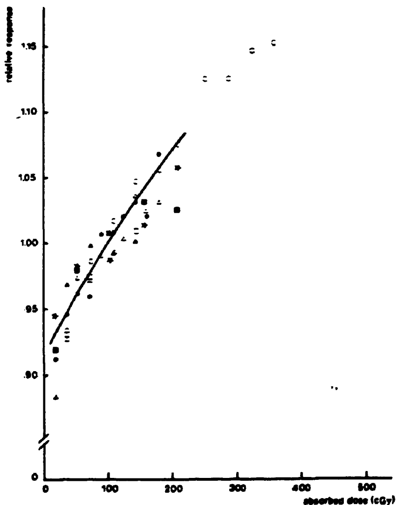
Fig. 1 Supralinearity of the response of LiF TLD-100 rods as a function of absorbed dose. The different symbols indicate different series of experiments employing different read-out and anneal procedures using equipment from different institutions.
