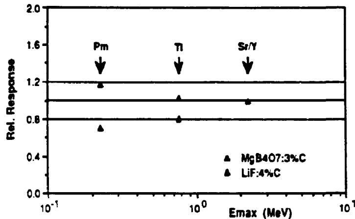
Fig. 6. Relative response for H_{\beta}(0.07) to beta radiation at normal incidence of the TNO TLD equipped with carbon loaded TL-material
