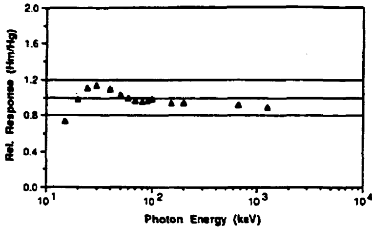
Fig. 4. Relative response for dose equivalent, superficial, of the TNO TLD badge
