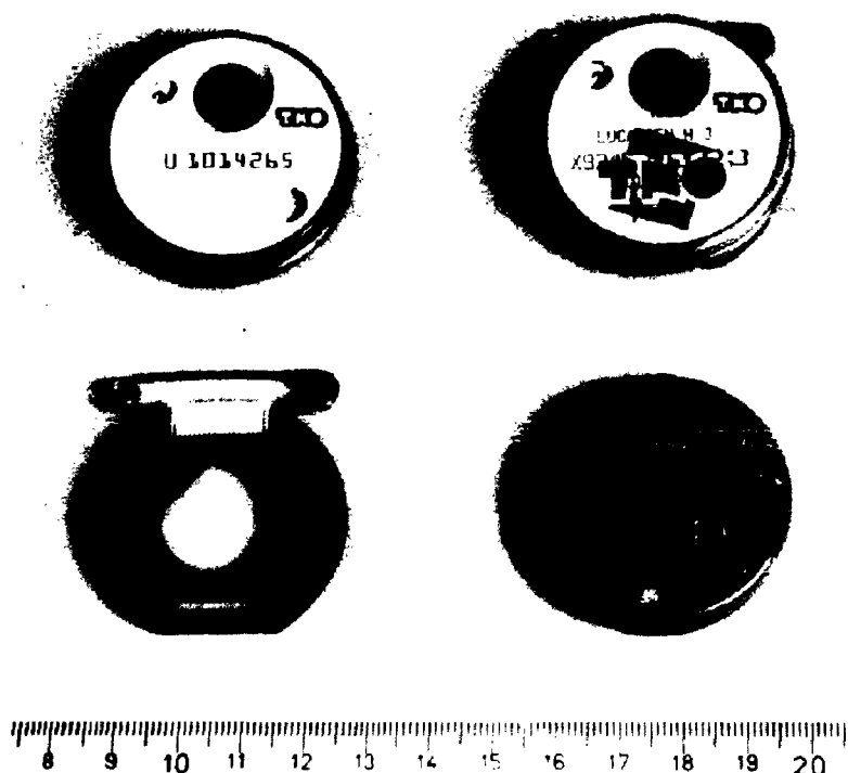
Fig. 3. The TNO TLD dosimeter, with and without the wearer's label, showing the individual's name, number and issuing period
