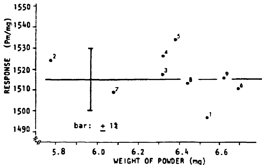
Fig. 2. Response in Pm/mg versus the weight of powder. The unit Pm stands for "Pitman", an apparatus bound arbitrary unit for response.
