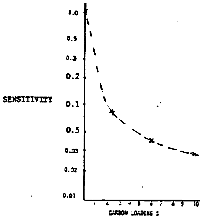
Fig. 1. Variation in sensitivity of disc with carbon loading (% by weight)
