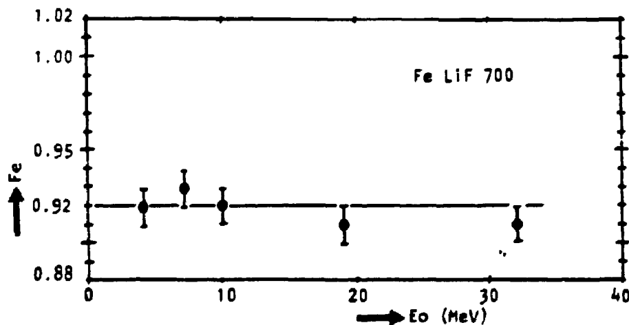
Fig. 2. Results of F_e measured with LiF 700 powder. Symbols are F_e determined using the NACP parallel-plate ionization chamber.
