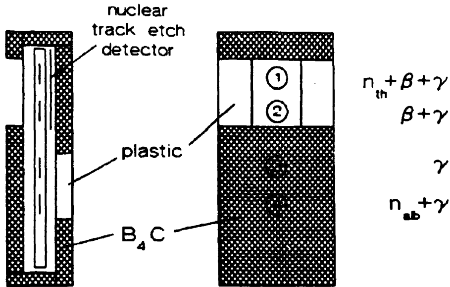
Figure 1. Construction of the dosimeter
