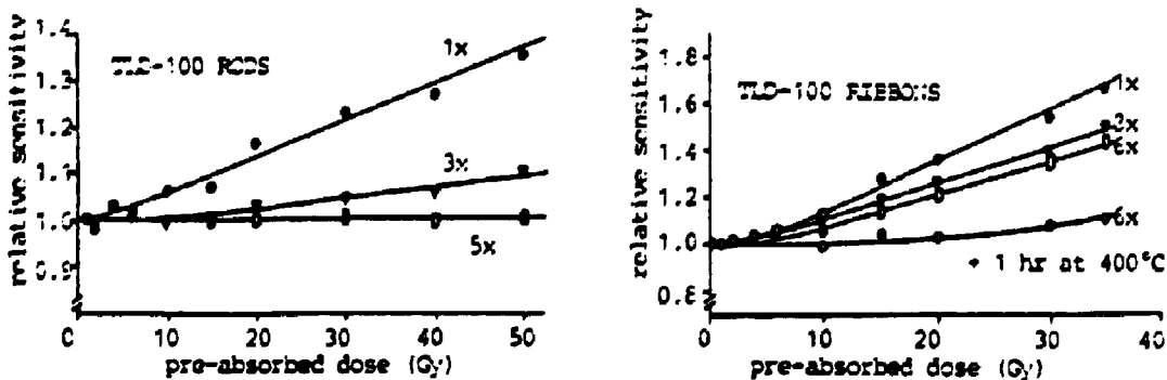
Fig. 2a and 2b. Relative sensitivity (normalized to and measured at 1 Gy) as a function of pre-irradiation dose and number of annealings.
