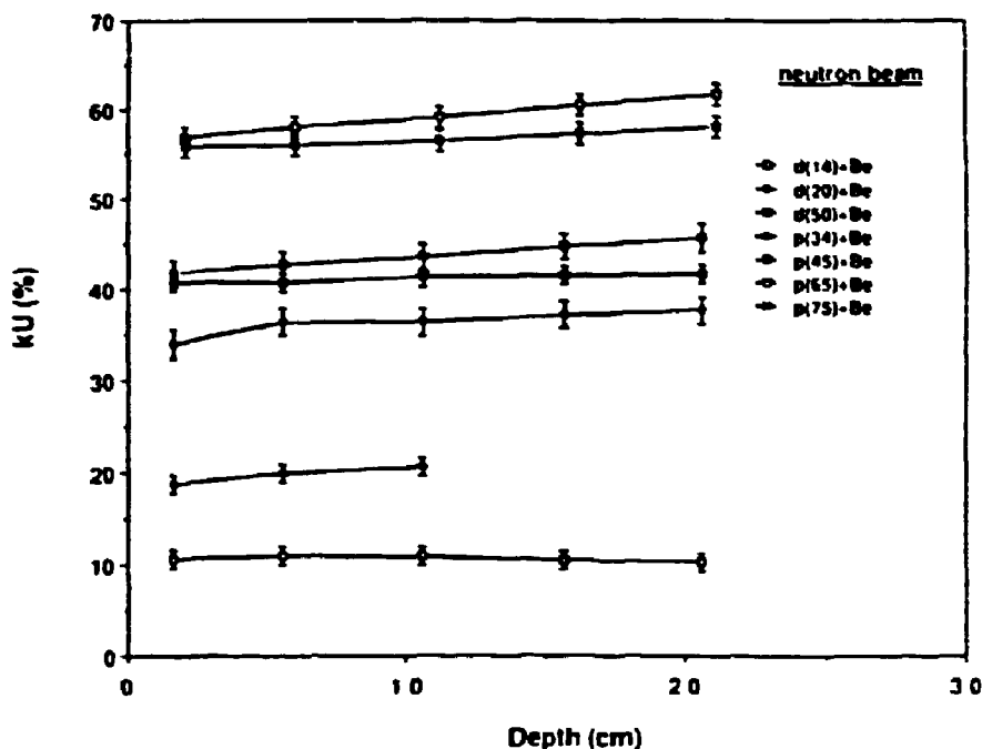
Fig. 3 : Variation of the k_U value of TLD700 as a function of the depth in a polystyrene phantom (10cm x 10cm field size).
