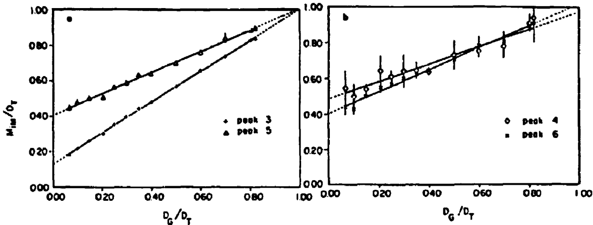
Fig. 2. Normalized TL-response as a function of the relative absorbed gamma dose of \text{CaF}_2:\text{Tm} (TLD-300) for (a) peak 3 and 5 and (b) for peaks 4 and 6. The straight lines are the result of a linear regression. The points are averages of four measurements with error bars of \pm one standard deviation.
