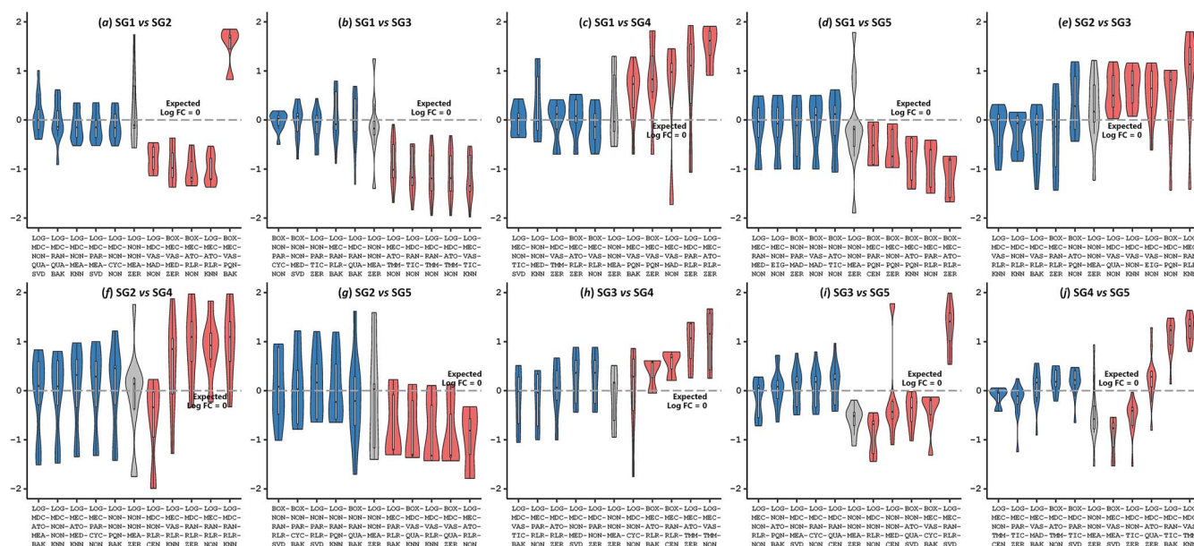
Figure 2. Accuracies of representative LFQ chains that were assessed using five SGs of various spiking protein concentrations. (A) SG1 versus SG2, (B) SG1 versus SG3, (C) SG1 versus SG4, (D) SG1 versus SG5, (E) SG2 versus SG3, (F) SG2 versus SG4, (G) SG2 versus SG5, (H) SG3 versus SG4, (I) SG3 versus SG5 and (J) SG4 versus SG5. All samples in each group were collected from the benchmark PXD014956 [30]. The horizontal dashed line represented an expected logFC of zero (completely consistent with spiking proteins). Violin plots in GRAY indicated the LFQ chain that was adopted in the original publication of the benchmark PXD014956 [30]. As illustrated, there are chances to identify an LFQ chain of better performance than the original one (colored in dark blue), and there are still great probabilities to discover the LFQ chain of much worse performance than the original one (colored in red). The abbreviations in each LFQ chain are explicitly described in Table 1.
