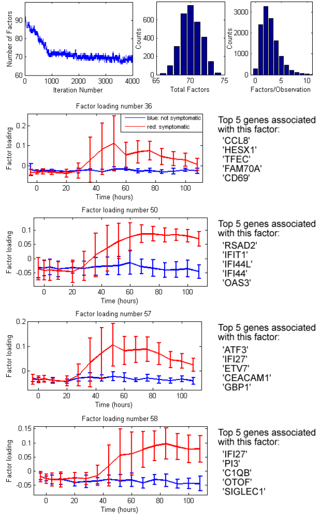
Figure 3. Results for time-evolving gene expression data. Top row: (left) Number of factors per iteration (middle) Histogram of the total number of factors after 1000 burn-in iterations (right) Histogram of the number of factors used per observation. Rows 2-5: Discriminative factors and the names of the most important genes associated with each factor (as determined by weight).
