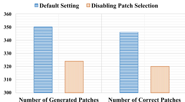
Fig. 3. Impact of patch selection.
