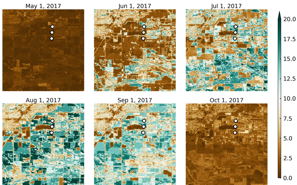
600 Figure A4. Examples of daily GPP ( \text{GC m}^{-2} \text{d}^{-1} ) derived from BESS-STAIR at Rosemount ( 44.65^\circ\text{N} - 44.75^\circ\text{N} , 93.05^\circ\text{W} - 93.15^\circ\text{W} ) in 2017. Circles indicate flux towers in this region.
