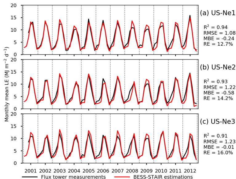
Figure A1. Time series of monthly mean ET from flux tower measurements and BESS-STAIR estimations.
