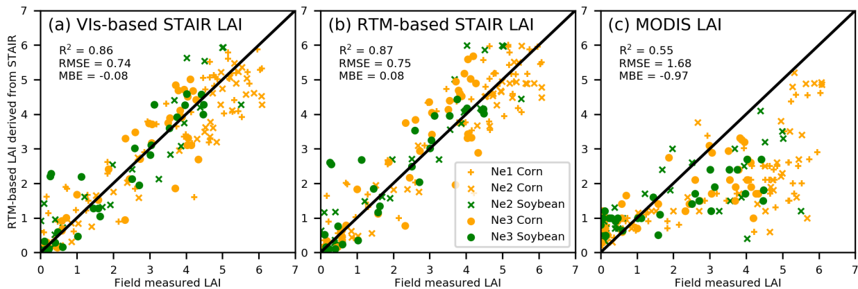
Figure 3. Scatter plots between LAI measurements and LAI estimations. LAI measurements are destructively collected at 315 three Mead sites. (a) – (b) STAIR-derived daily 30m-resolution LAI using VIs-based method and RTM-based method, respectively. (c) 500m-resolution MODIS LAI.
