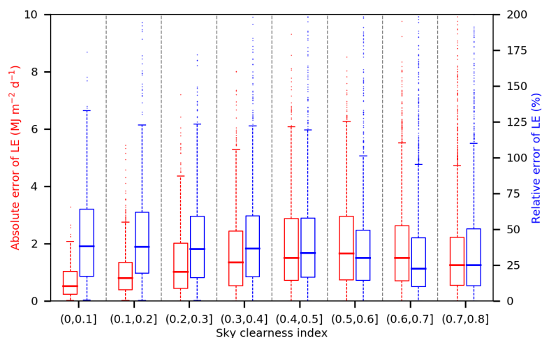
Figure 12. BESS-STAIR estimated daily ET has similar performance with varying sky clearness index (the ratio of incoming radiation on surface to that on top-of-atmosphere). The lower and upper boundaries of boxes refer to the first and third 490 quartile of error statistics. The bars inside boxes refer to median values. The whiskers indicate 1.5 times of distance between the first and third quartiles.
