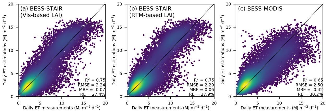
Figure 4. Density scatter plots between ET measurements and ET estimations. ET measurements are from eddy covariance data collected at 12 flux towers. (a) and (b) BESS-STAIR ET with Vis-based LAI and RTM-based LAI, respectively. (c) 500m-BESS ET with MODIS LAI.
