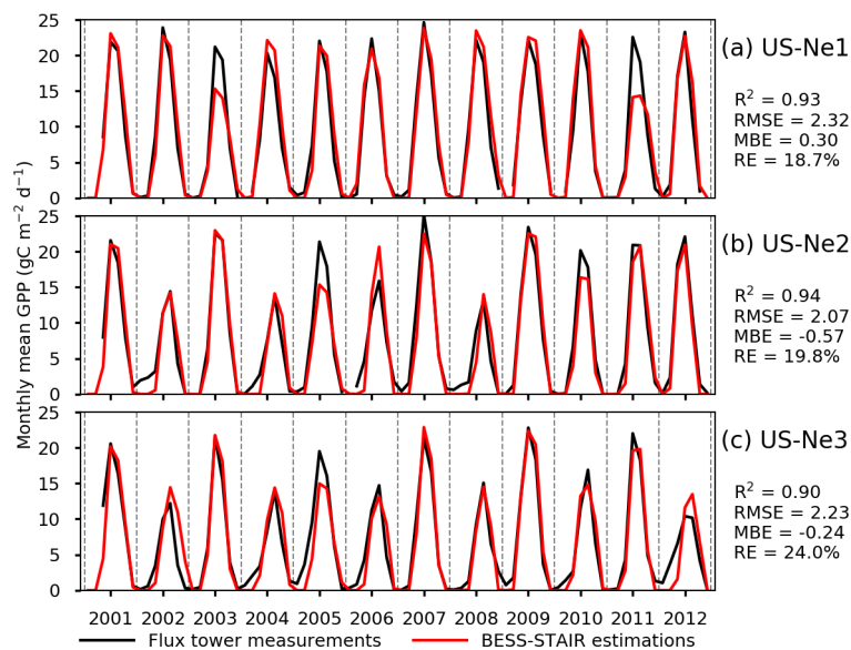
Figure A2. Time series of monthly mean GPP from flux tower measurements and BESS-STAIR estimations. Significant underestimations in 2003 and 2011 for Ne1, in 2005 for Ne2, and in 2005 for Ne3 are due to misclassification of corn as soybean in CDL. Significant overestimations in 2006 for Ne2 are due to misclassification of soybean as corn in CDL.
