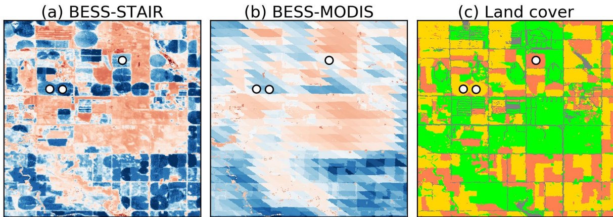
Figure 8. Daily ET ( \text{MJ m}^{-2} \text{d}^{-1} ) derived from (a) BESS-STAIR and (b) BESS-MODIS at Mead ( 41.1^\circ\text{N} - 41.2^\circ\text{N} , 96.4^\circ\text{W} - 96.5^\circ\text{W} ) on August 1, 2012. Circles indicate flux towers in this region.
