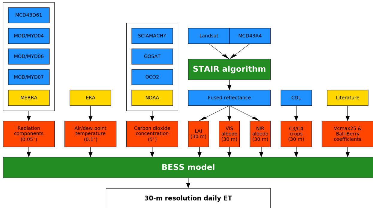
Figure 1. The BESS-STAIR framework. The BESS ET estimation model and the STAIR data fusion algorithm are 115 highlighted in green boxes. Blue boxes are satellite data, yellow boxes are ancillary data, and red boxes are key inputs to BESS. The output of BESS-STAIR is the 30-m resolution daily ET highlighted in white box.
