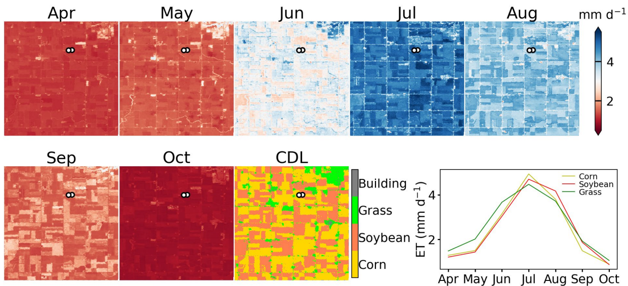
380 Figure 9. Monthly mean BESS-STAIR ET at Brooks Field (41.9°N – 42.0°N, 96.65°W – 96.75°W) during the growing season of 2000, along with a CDL land cover map. The last subplot shows the average time series of corn, soybean and grass. Circles indicate flux towers in this region.
