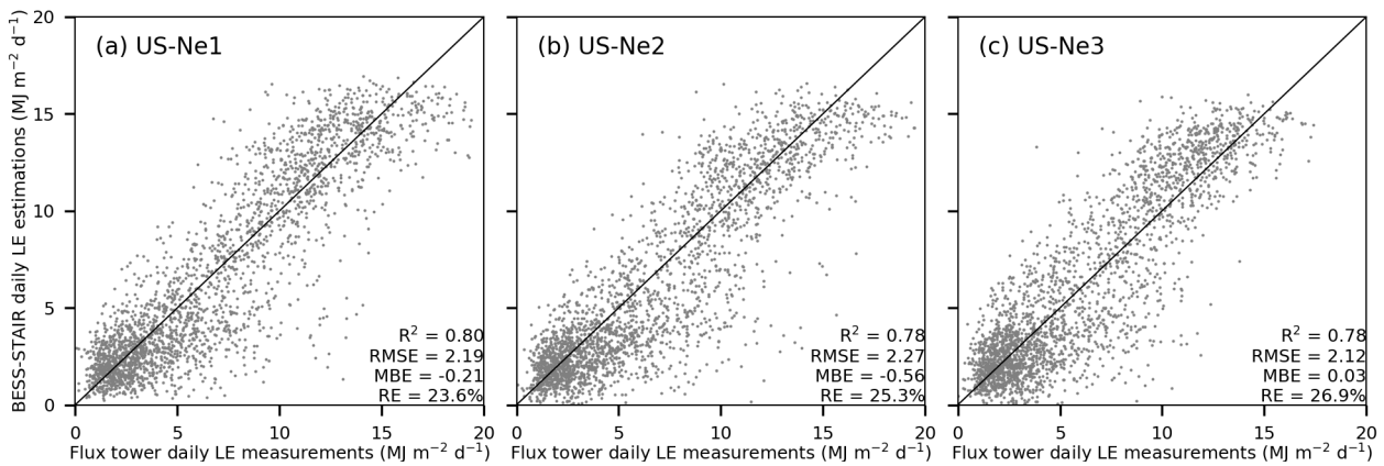
435 Figure 11. Scatter plots between ET measurements and ET estimations at three sites US-Ne1, US-Ne2 and US-Ne3.
