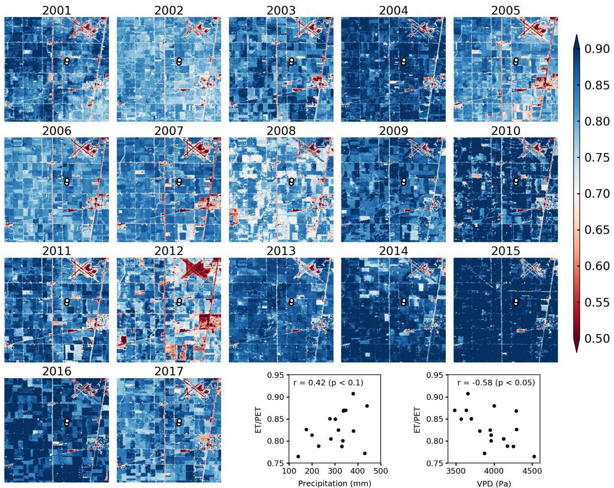
Figure 10. Peak growing season (June, July and August) BESS-STAIR ET/PET at Bondville (39.95°N – 40.05°N, 88.25°W – 88.35°W) from 2001 throughout 2017, along with two scatter plots between peak growing season precipitation and ET/PET and peak growing season VPD and ET/PET over the 17 years. Precipitation and VPD data are from Daily Surface Weather Data (Daymet) at Illinois Bondville ( https://modis.ornl.gov/cgi-bin/sites/site/?id=us_illinois_bondville&product=Daymet ), where VPD is derived using maximum air temperature and water vapor pressure. Circles indicate flux towers in this region.
