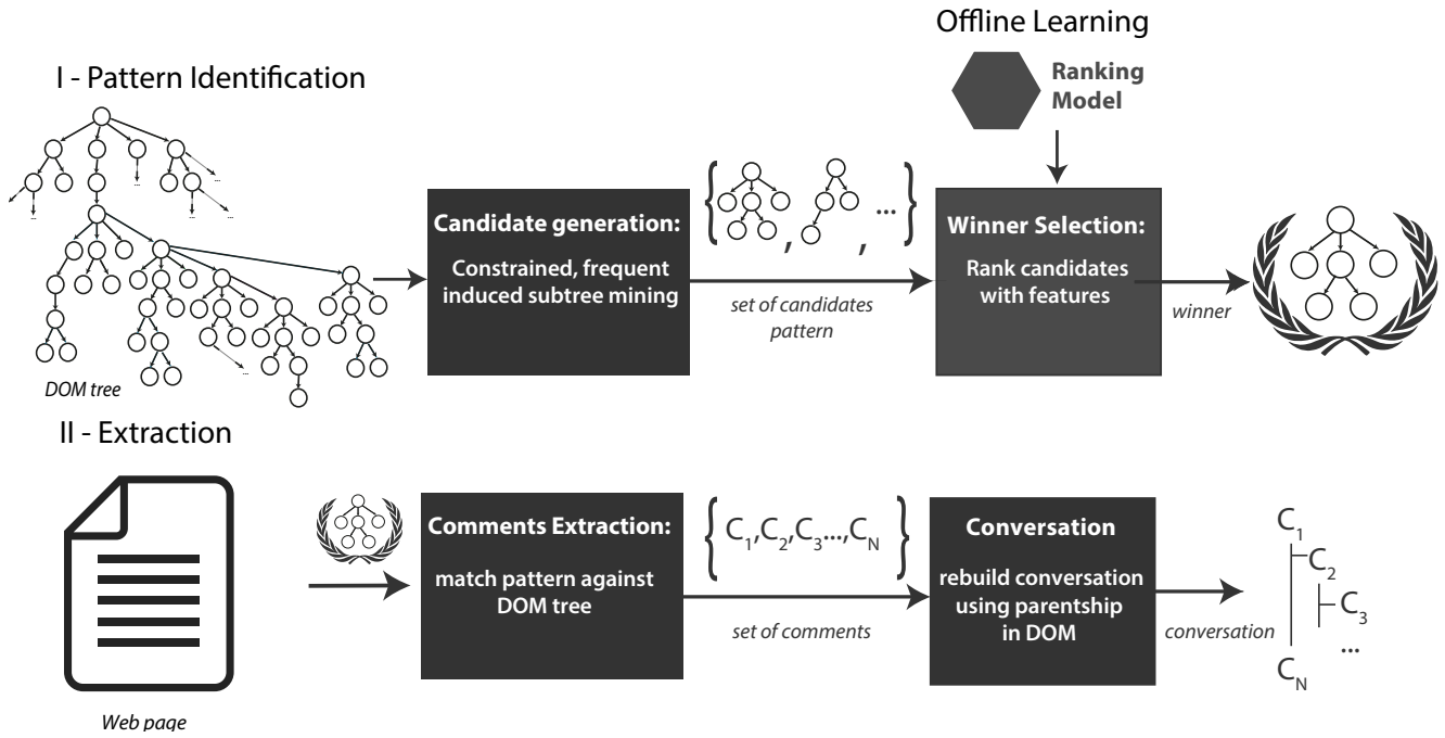
Fig. 2: Outline of CommentsMiner
