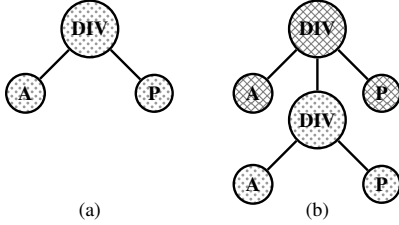
Fig. 4: Example of subtrees. The comment pattern is (A, P)DIV (in Newick tree format).
