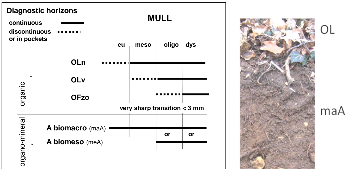
Fig. 10a. Terroforms, second level of classification of Mull. Lines: diagnostic horizons, sequence as in real profile. Columns: second level of classification. Names of second level of Mull forms: eumull, mesomull, oligomull, dysmull.
