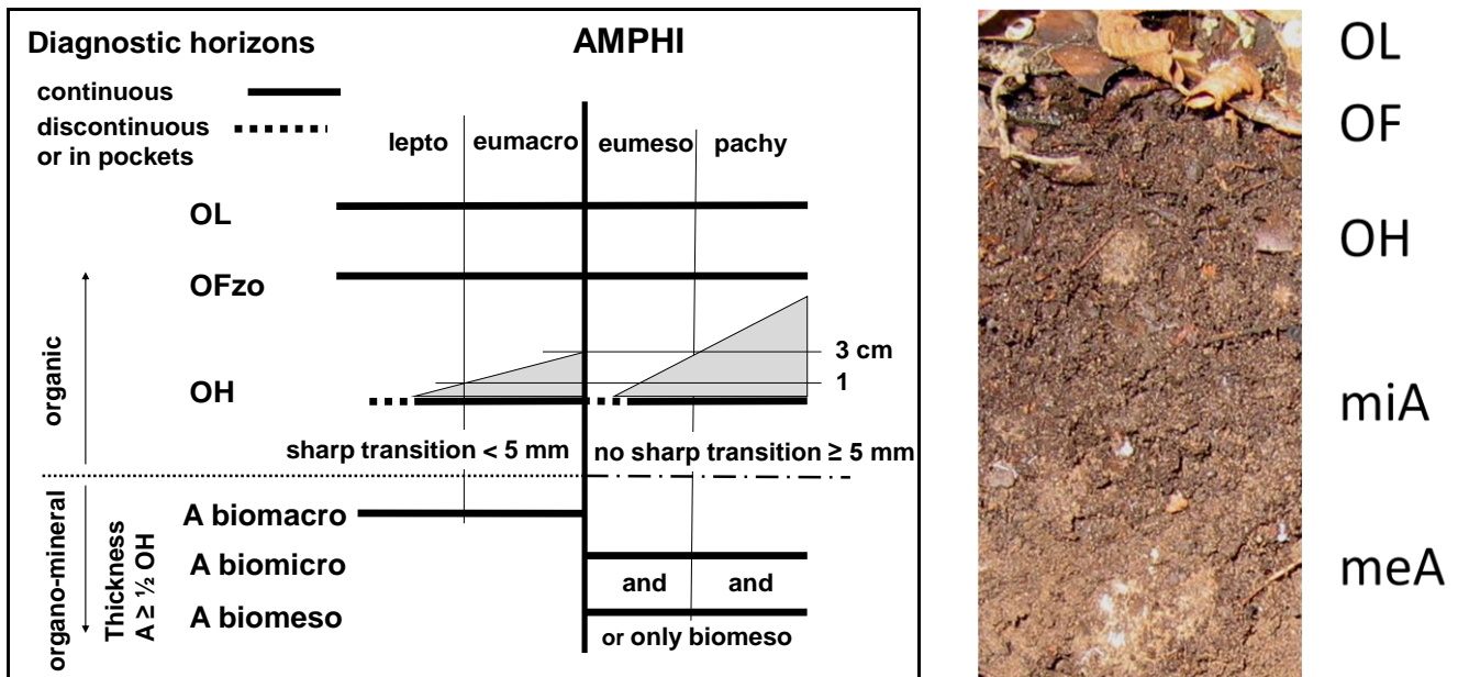
Fig. 10b. Terroforms, second level of classification of Amphi. Lines: diagnostic horizons, sequence as in real profile. Columns: second level of classification. Names of second level of Amphi forms: lepteamphi, eumacroamphi, eumesoamphi, pachyamphi.
