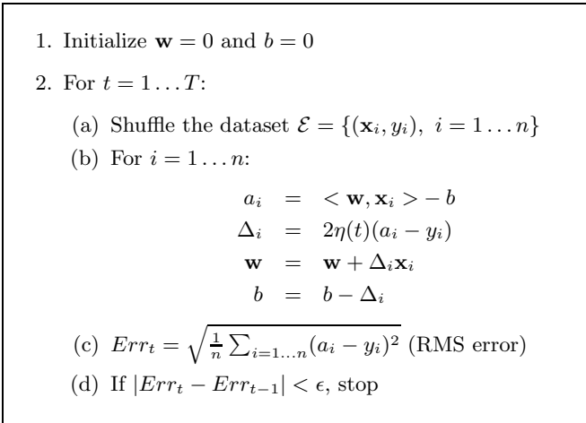
Figure 3: Least-mean square training algorithm.
