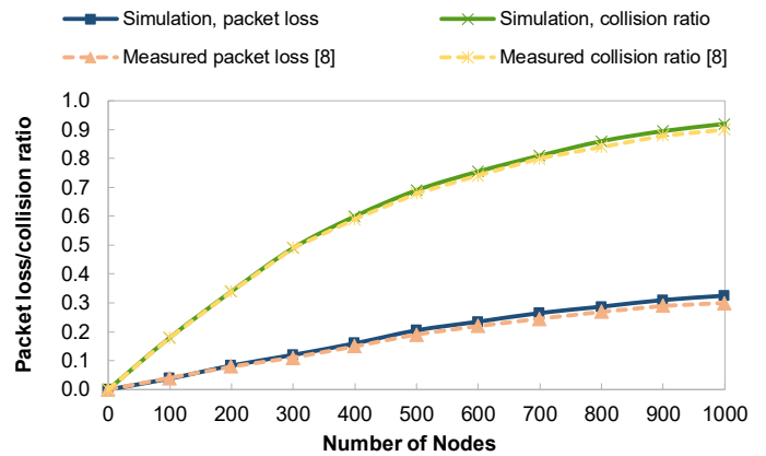
Fig. 5: Comparison between simulated values and measurements by Haxhibeqiri et al. [8] showing the impact of the capture effect.
