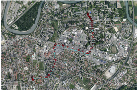
Fig. 2: The real environment for deployment the testbed. The distance from end devices to the gateway is increased gradually.
