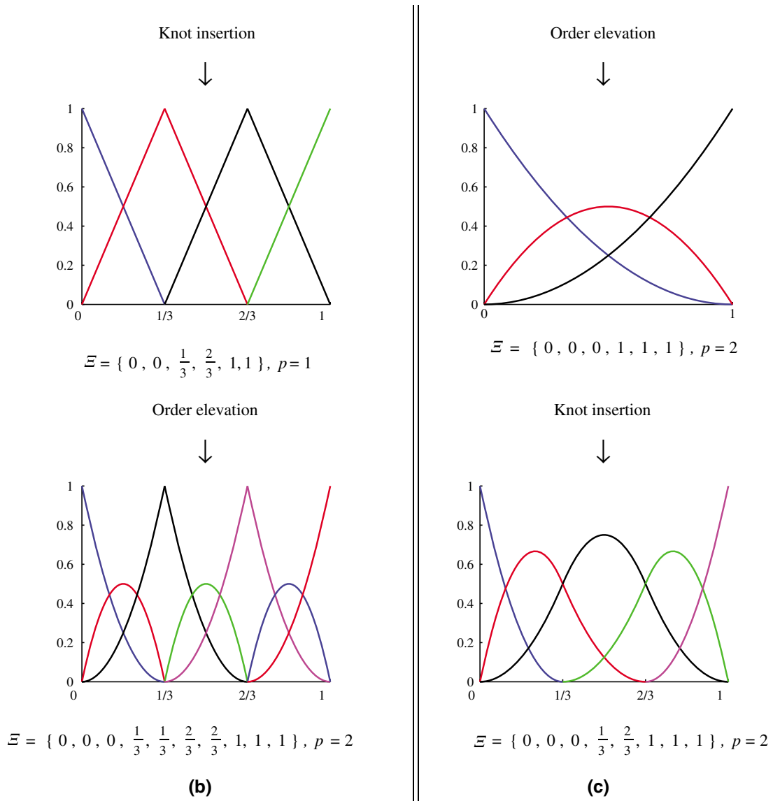
Fig. 10. k -refinement takes advantage of the fact that knot insertion and order elevation do not commute. (a) Base case of one linear element. (b) Classic p -refinement approach: knot insertion followed by order elevation results in seven piecewise quadratic basis functions that are C^0 at internal knots. (c) New k -refinement approach: order elevation followed by knot insertion results in five piecewise quadratic basis functions that are C^1 at internal knots.
