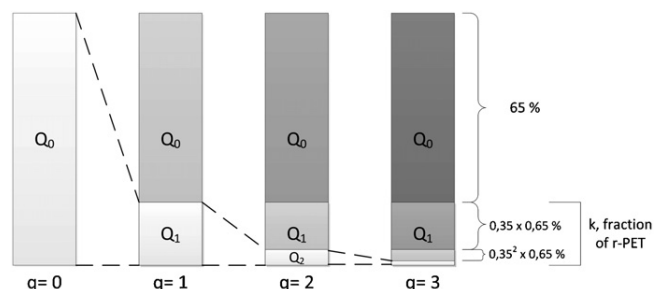
Fig. 18. Mix of resins in a PET bottle. Q_n represents the quality, linked to the number of times this fraction has been recycled, Q_0 being virgin PET and q the number of recycling trips.
