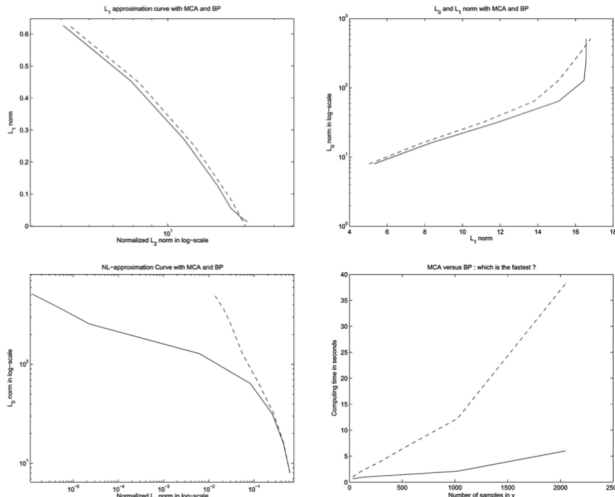
Fig. 5. Top left: l_1/l_2 -curve of both (solid line) MCA/MOM and (dashed line) BP. Top right: l_0/l_1 -curve of both (solid line) MCA/MOM and (dashed line) BP. Bottom left: Nonlinear approximation curve ( l_0/l_2 ) of both (solid line) MCA/MOM and (dashed line) BP. Bottom right: Comparison of execution times (in seconds): (solid line) MCA/MOM and (dashed line) BP.
