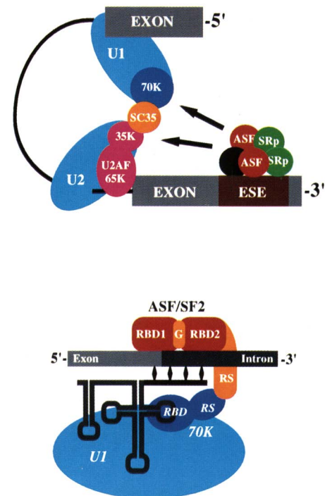
Figure 2. SR proteins are involved in various steps of spliceosome assembly. (Top) ASF/SF2 and SC35 connect 5' and 3' splice site complexes through a network of protein–protein interactions (see text for detail). Activation of splicing of weak introns by exonic splicing enhancer (ESE) elements requires sequence-specific binding of SR proteins (SRp) such as ASF/SF2 (ASF), and other nuclear factors, such as, for example, Tra2 (black circle), to the ESE. SR proteins help to connect the enhancer complex to the 5' and/or 3' splice site via protein–protein interactions with U1 70K and/or U2AF 35 (arrows), thereby facilitating or stabilizing binding of U1 and/or U2 snRNPs. SC35, and perhaps other SR proteins, may also function to bridge the U1 and U2 snRNP complexes. (Bottom) SR proteins such as ASF/SF2 recruit U1 snRNP to and/or stabilize its interaction with the 5' splice site. ASF/SF2 binds at or near the 5' splice site via its RBDs, while its RS domain interacts with the RS region in the U1 70K protein. 70K is in turn bound via its own RBD to the first stem–loop of U1 snRNA, and the 5' end of U1 snRNA base pairs with the 5' splice site. Note that the mechanism by which the two RBDs of ASF/SF2 cooperate in RNA recognition is not known, nor is it clear that the RS regions of the two proteins, although necessary for association, interact directly.
