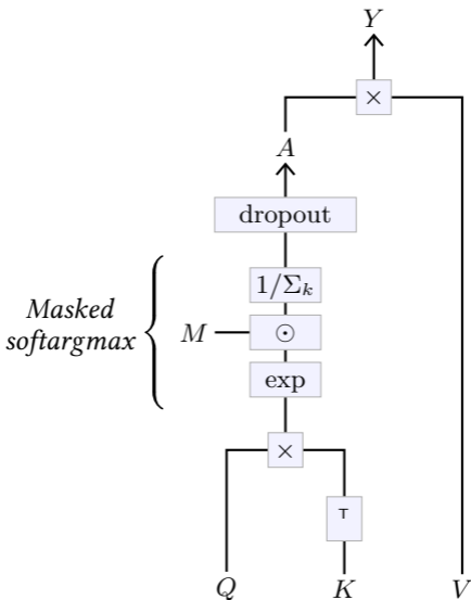
Figure 4.12: The attention operator Y = \text{att}(Q, K, V) computes first an attention matrix A as the per-query softargmax of QK^T , which may be masked by a constant matrix M before the normalization. This attention matrix goes through a dropout layer before being multiplied by V to get the resulting Y . This operator can be made causal by taking M full of 1s below the diagonal and zeros above.
