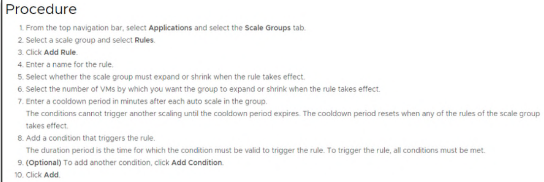
13 Figure 40. Screenshot showing procedure for auto-scaling in VMware Cloud Director. 122
