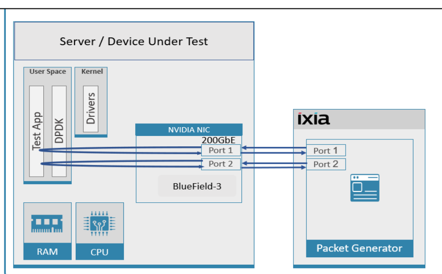
Figure 23: Test #12 Setup – NVIDIA BlueField-3 2x200GbE connected to IXIA
