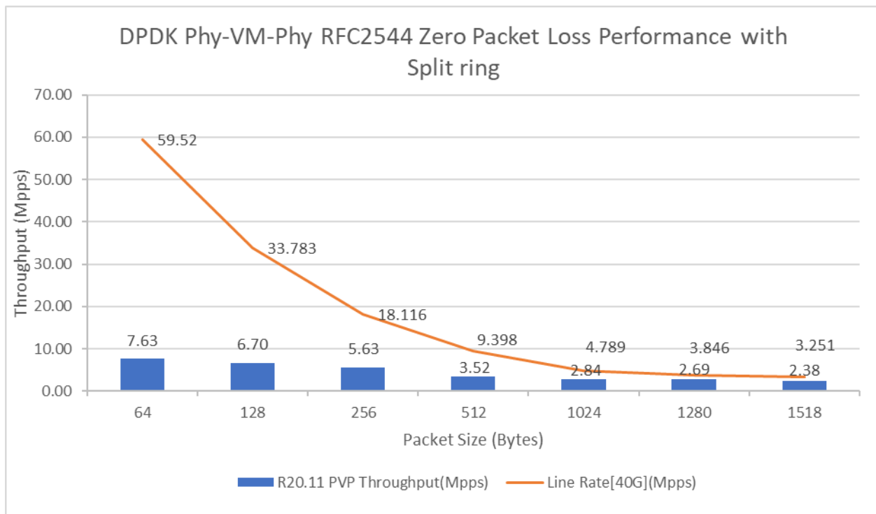
Figure3. RFC2544 zero packet loss performance with Split ring Vhost/Virtio PVP Mergeable
