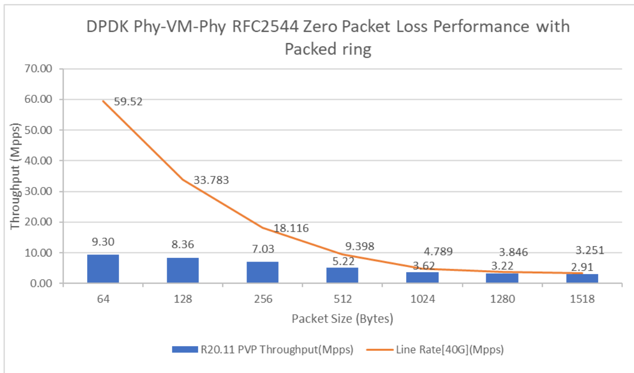
Figure4. RFC2544 zero packet loss performance with Packed ring Vhost/Virtio PVP Mergeable
