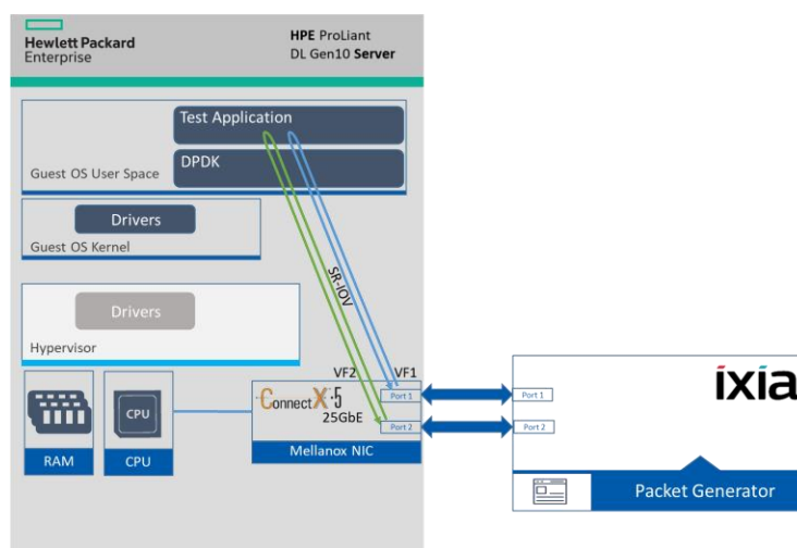
Figure 13: Test #7 Setup – Mellanox ConnectX-5 25GbE connected to IXIA using ESXi SR-IOV
