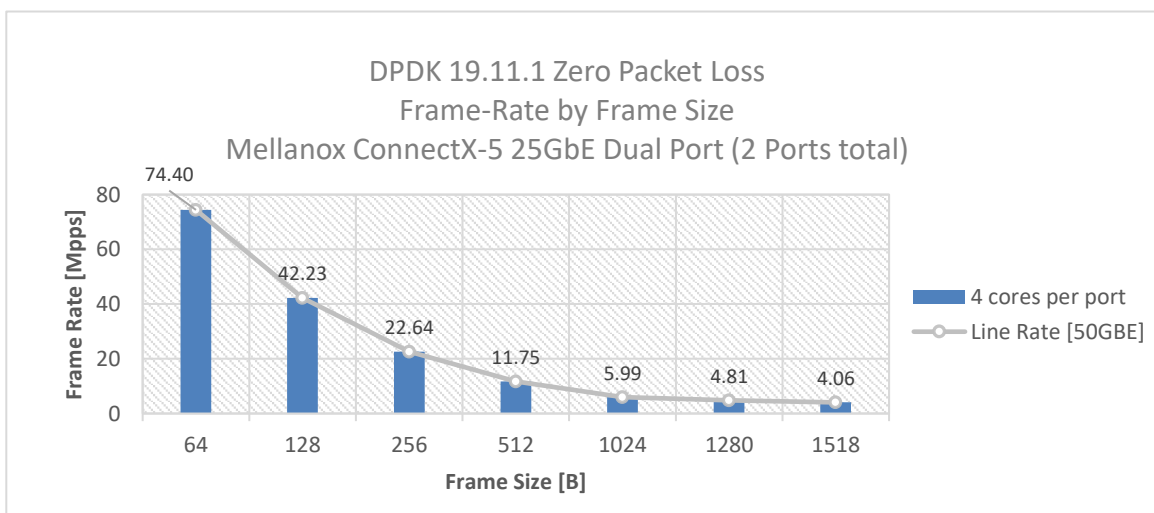
Figure 4: Test #2 Results – Mellanox ConnectX-5 25GbE Dual-Port Throughput at Zero Packet Loss
