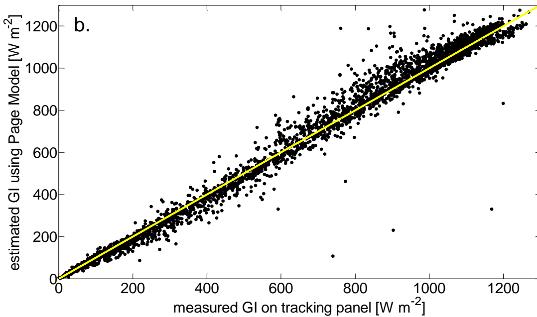
Figure 1: Scatter plot of (a) the measured GI on a surface at 40^\circ tilt, facing due south, and (b) the measured GI on a tracking panel, plotted versus values calculated using the Page Model. Measurements were taken at SRRL in Golden, Colorado. The values shown are hourly daytime values (solar elevation angle >10^\circ ) for the entire year 2009. The solid lines are 1:1 lines for reference.
