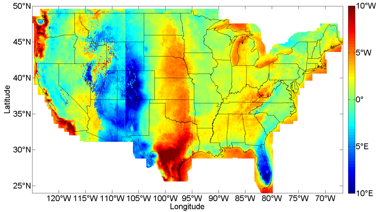
Figure 3: Map showing the optimum azimuth to maximize incident GI. Due south is 0^\circ , and values shown on the map are east or west of due south. When coupled with Figure 2a, the optimum orientation (tilt and azimuth) at any location on the map can be determined.
