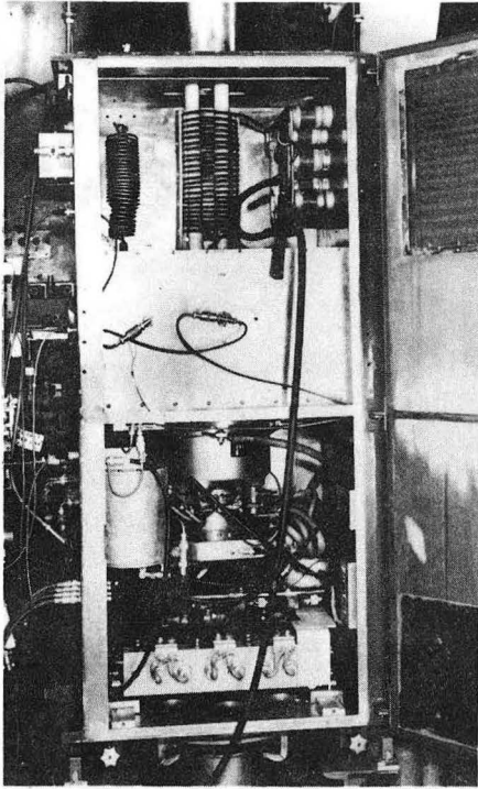
Figure 1. Front View of P.A. Cabinet
