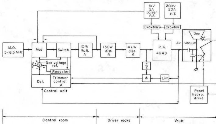
Figure 4. Block Diagram
