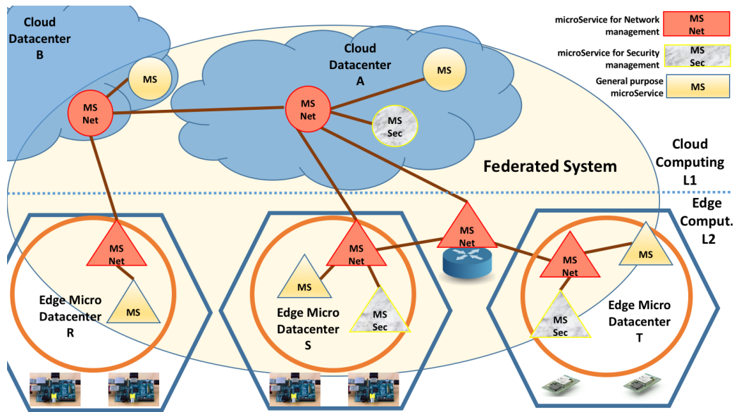
Fig. 4: A two Layer (L1/L2) Federated Cloud Environment in Osmotic Computing .
