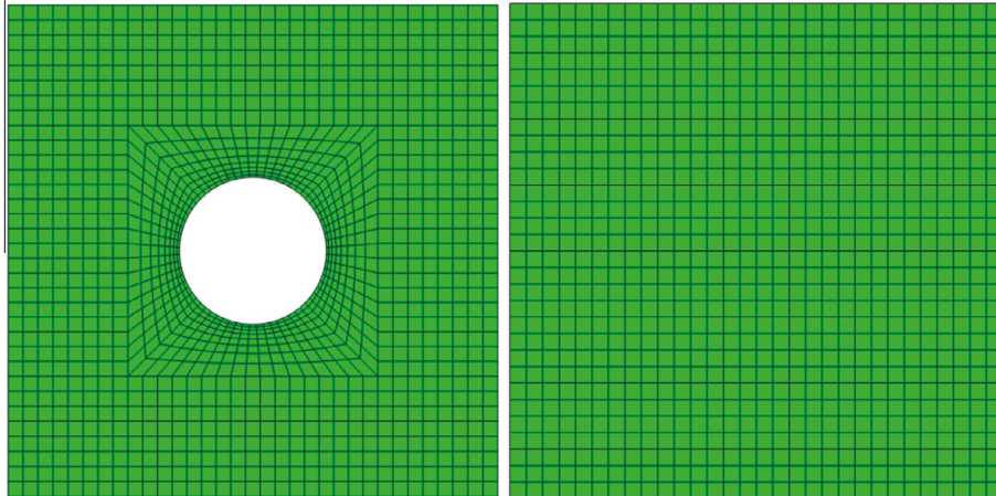
Fig. 5. Discretization of notched and un-notched laminates.
