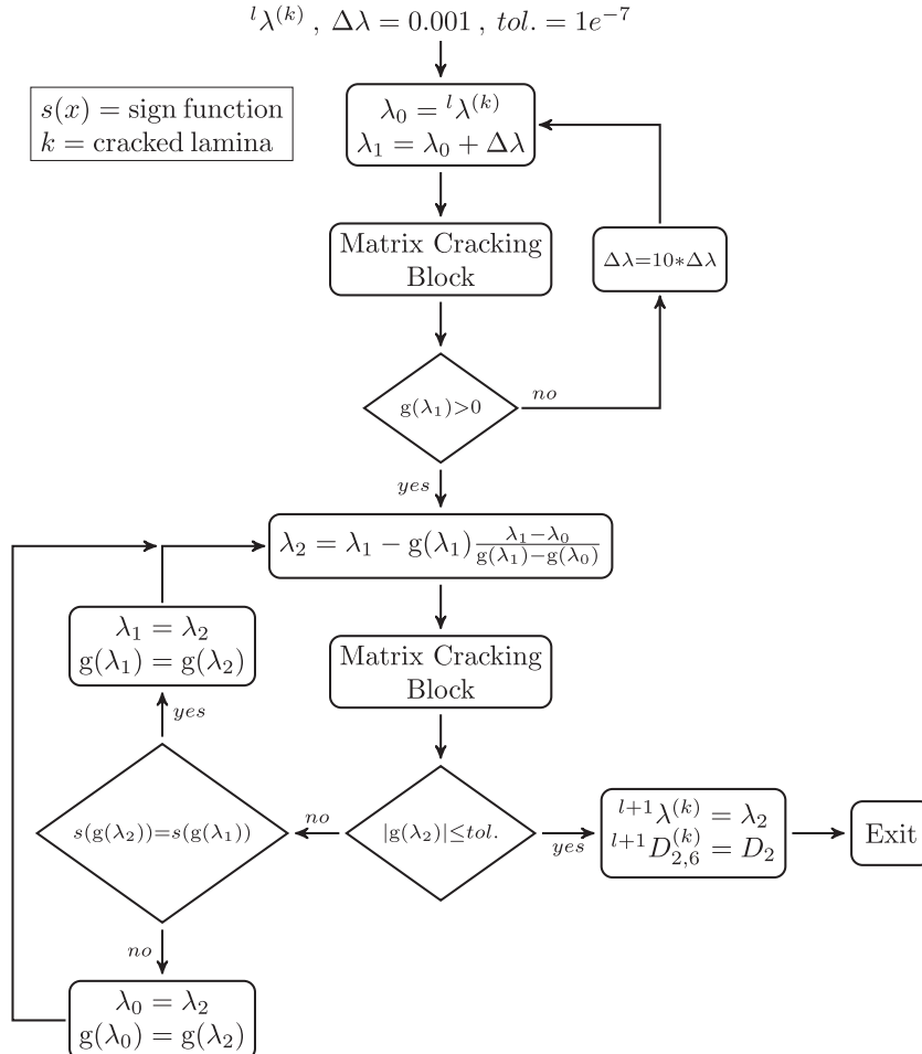
Fig. 3. Regula Falsi algorithm implemented.
