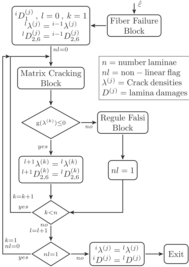
Fig. 4. Laminate implementation scheme of the combined formulation.
