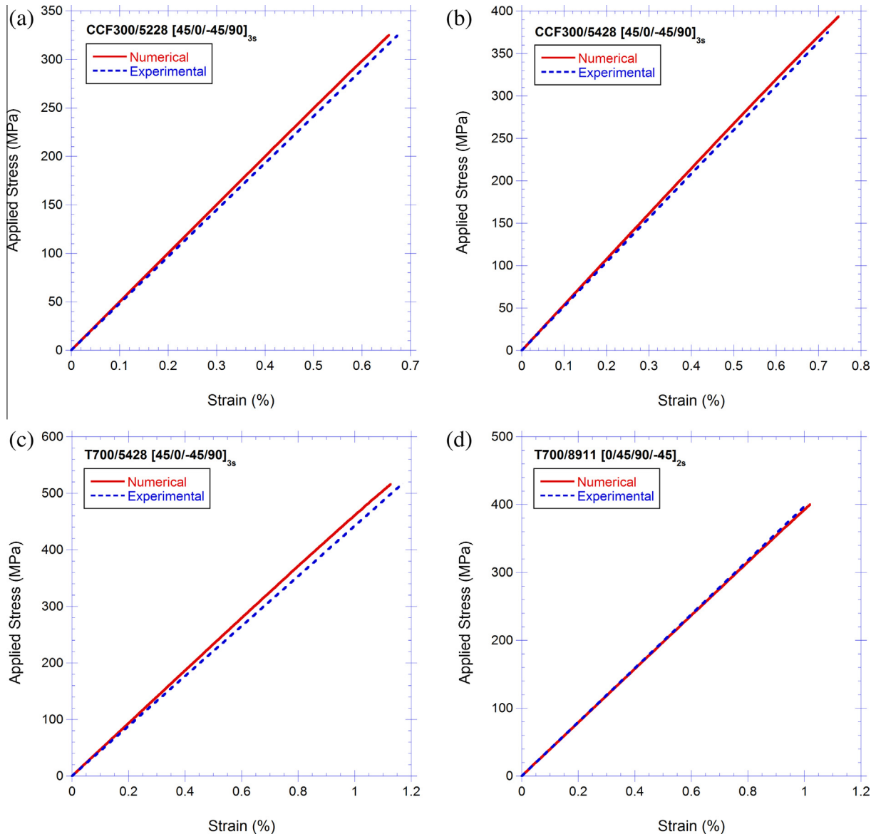
Fig. 7. Comparison between numerical and experimental applied stress–strain curve for: (a) CCF300/5228 [8], (b) CCF300/5428 [8], (c) T700/5428 [8] and (d) T700/8911 [16].
