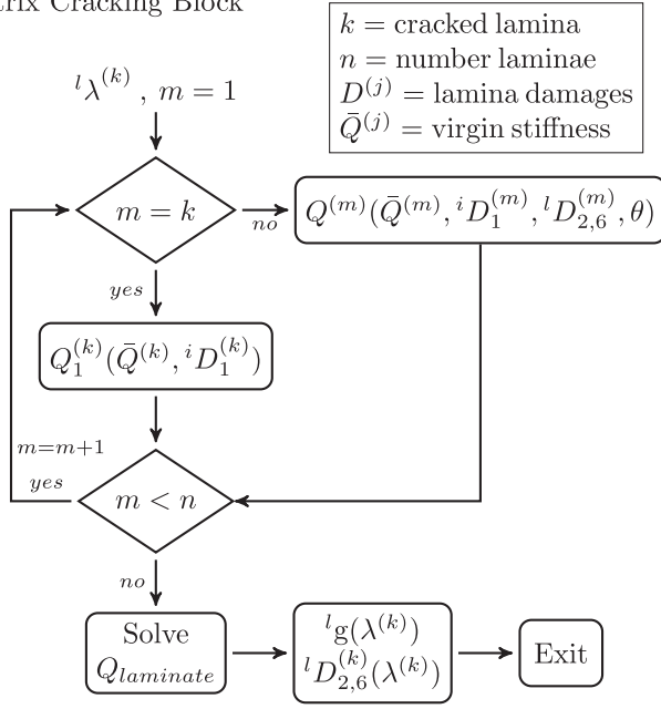
Fig. 2. Matrix cracking implementation.
