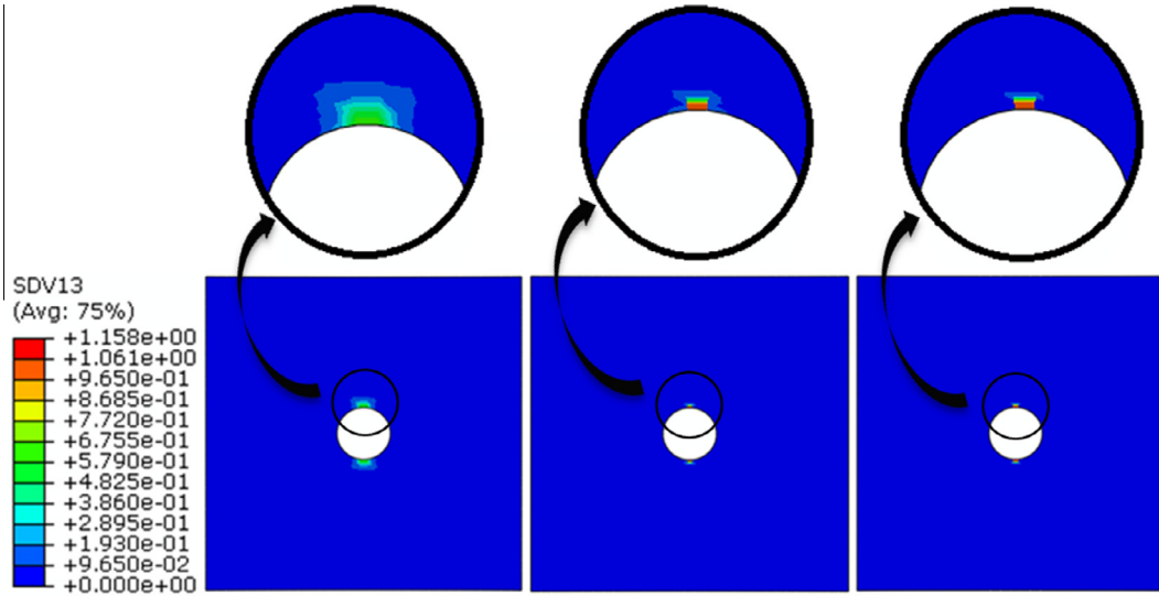
Fig. 9. Longitudinal damage on 0° plies for different values of m (3, 5 and 7 from left to right).
