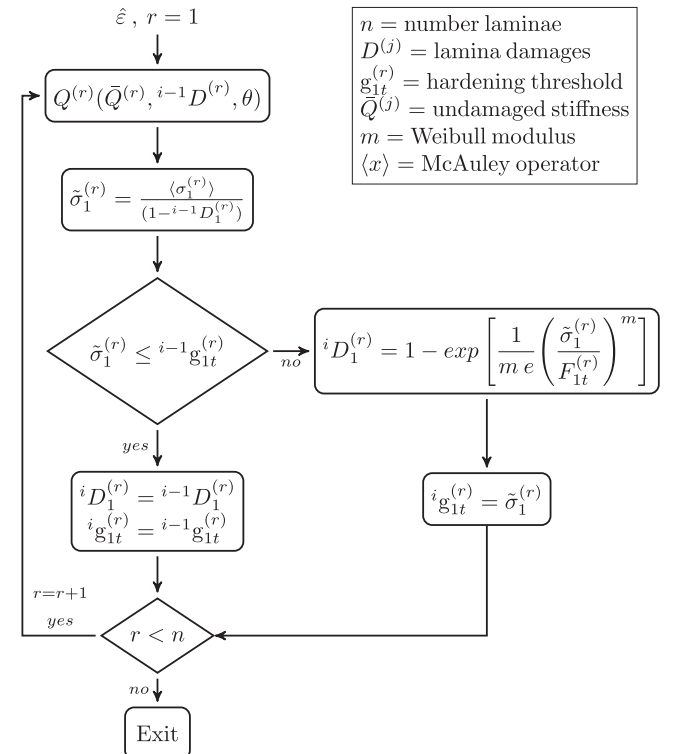
Fig. 1. Fibre failure algorithm scheme.
