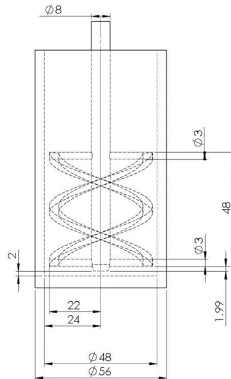
Figure 30. A design drawing for a proposed “double-helix” rheometer blade.
