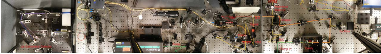
Figure 48. Experimental setup for quantum repeater development.
