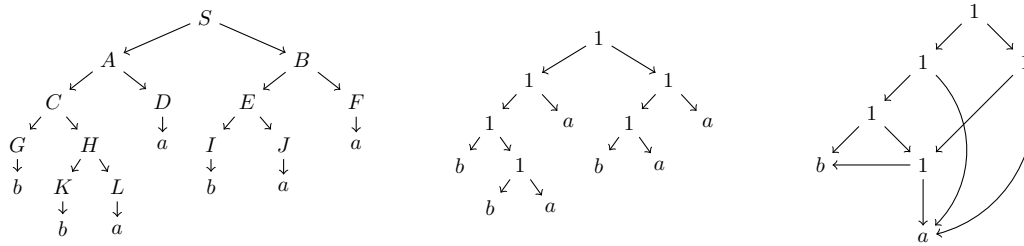
Figure 2 The derivation tree from Example 4.
