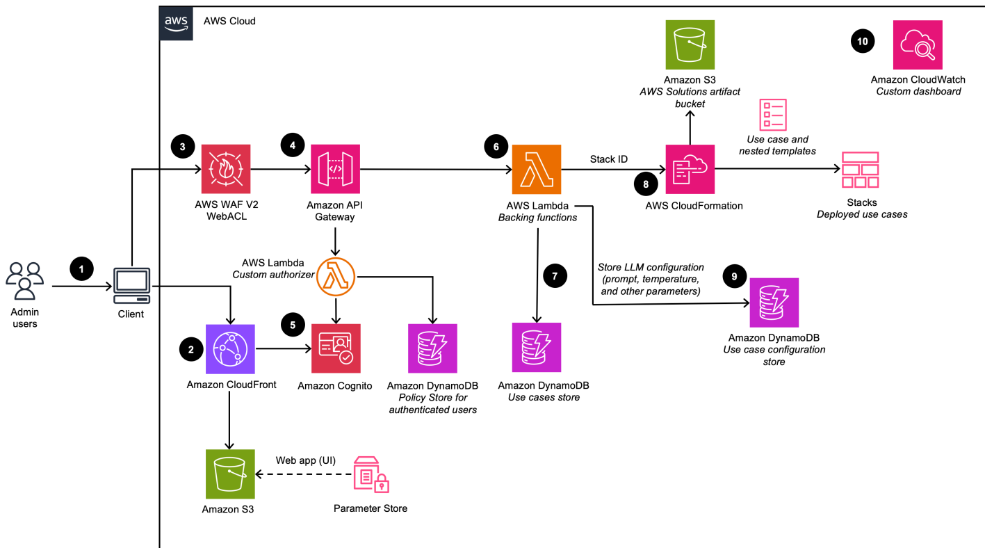
Deployment dashboard architecture (when deployed with VPC option disabled)
