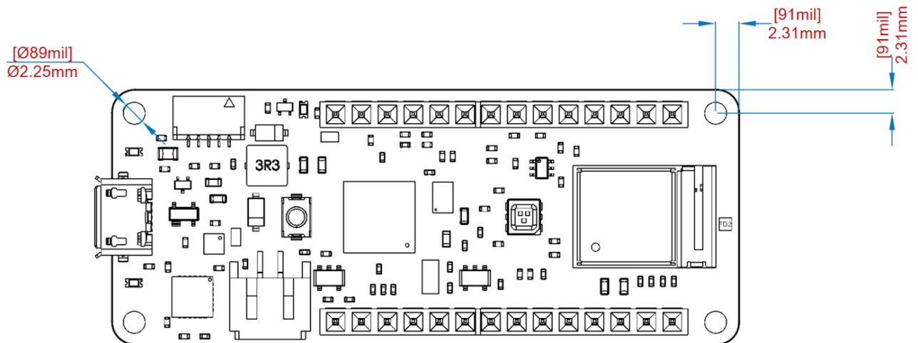
MKR WiFi 1010 Mounting Holes
