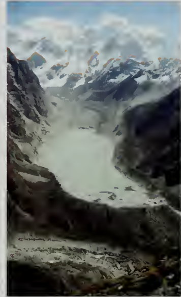
Tsho Rolpa, 4 580 m, the most studied glacial lake in Nepal, in October 2000. The lake formed at the head of the Rolwating Valley as the Trakarding Glacier retreated. It is dammed by an ice-cored moraine and now extends over 3 km and contains an estimated 80 million m 3 of water.
