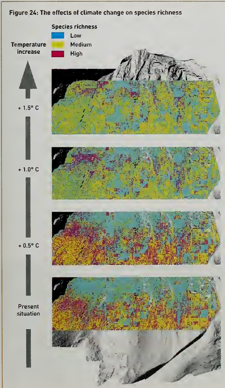
Figure 24: For 21 species studied, overall richness is currently greatest within the alpine-snowline transition zone, but computer models predict that richness will decline sharply with climate warming as different species become 'trapped' in particular terrain situations.
