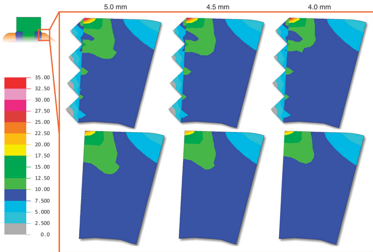
Figure 3. Oblique loading stress plots. Top row shows microthread model; bottom row shows smooth-neck model. Key shown in von Mises stress (MPa).
