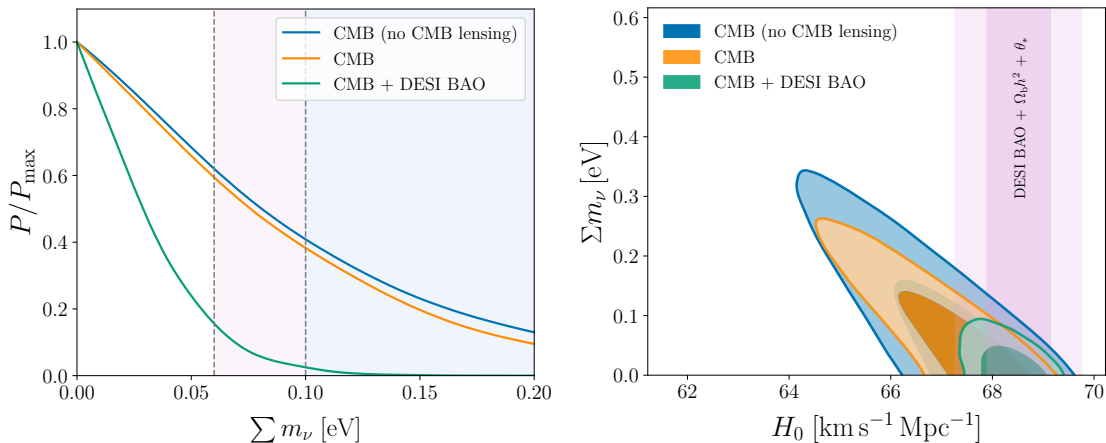
Figure 11. Left panel: The marginalized 1D posterior constraints on \sum m_\nu from different combinations of datasets, in the single parameter extension flat \Lambda CDM+ \sum m_\nu model. As explained in the text, here we use a model with 3 degenerate mass eigenstates and with a minimal prior \sum m_\nu > 0 eV. The minimal masses for the normal or inverted mass ordering scenarios correspond to \sum m_\nu > 0.059 eV and \sum m_\nu > 0.10 eV respectively, shown by the vertical dashed lines and the shaded regions. Right panel: Joint marginalized 68% and 95% credible intervals on \sum m_\nu and H_0 from Planck , CMB and DESI+CMB data, illustrating the degeneracy between these parameters from the CMB, and how DESI BAO data contribute to breaking it. The vertical shaded regions indicate the 68% and 95% constraints on H_0 from DESI BAO data combined with knowledge of \theta_* and \Omega_b h^2 in the \Lambda CDM+ \sum m_\nu model. This shows how DESI BAO breaks the primarily geometric degeneracy to place an upper limit on \sum m_\nu .
