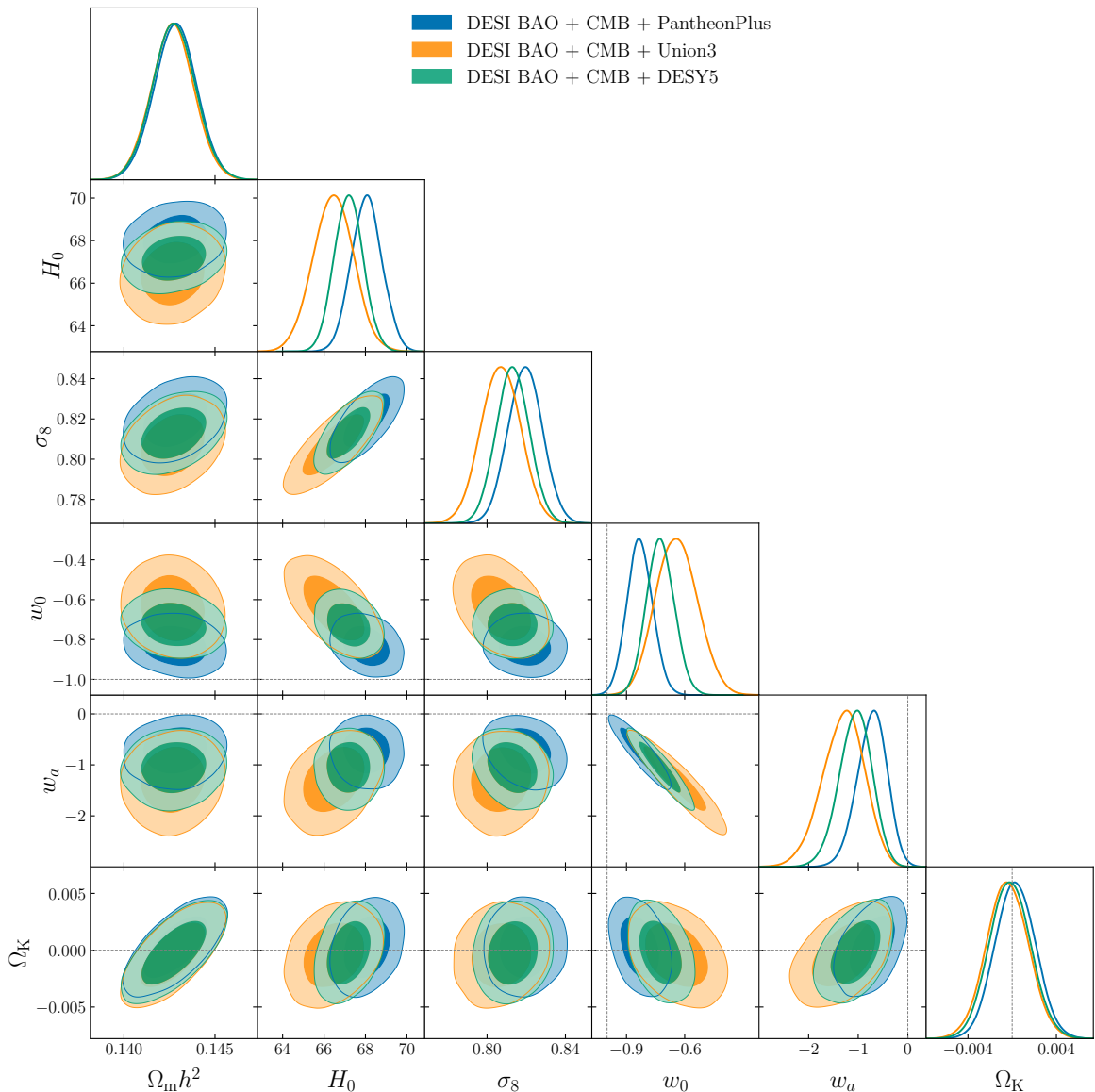
Figure 8. Marginalized posteriors on w_0 , w_a and \Omega_K in a model with a time-varying dark energy equation of state and free spatial curvature, from DESI and CMB data combined with SN Ia from PantheonPlus, Union3 and DESY5 in blue, orange and green respectively. All combinations provide tight limits on \Omega_K . Constraints on w_0 and w_a in each case broaden a little compared to those shown in the flat case (Figure 6) but the overall trend remains the same.
