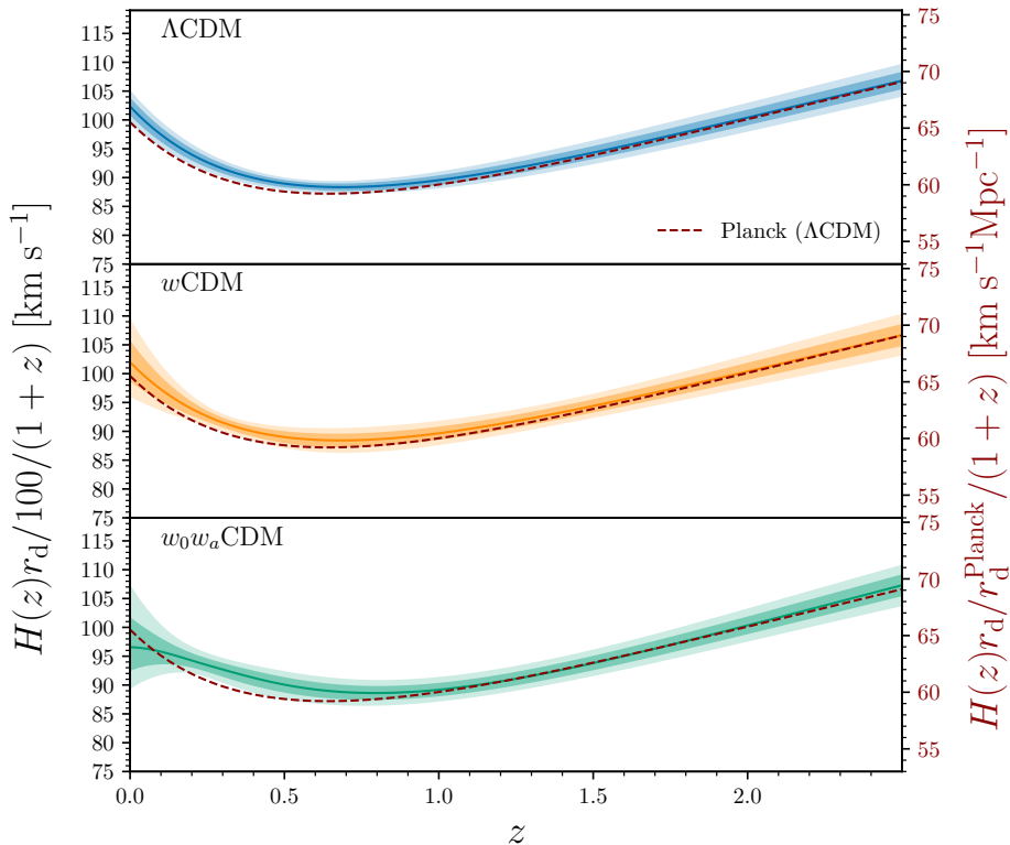
Figure 7. Model-dependent constraints on the redshift dependence of the Hubble parameter times the sound horizon, H(z)r_d \equiv r_d/D_H (scaled by 1/100/(1+z) for visual clarity) in three different classes of models fit to all DESI data from Figure 1. From top to bottom, the panels show the 68% and 95% credible regions in the \Lambda CDM, w CDM and w_0w_a CDM models respectively in the coloured bands. The dashed line in each panel shows the behaviour in the best fit Planck \Lambda CDM model. For convenience, the scale on the right-hand axis shows (r_d/r_d^{\text{Planck}})H(z)/(1+z) .
