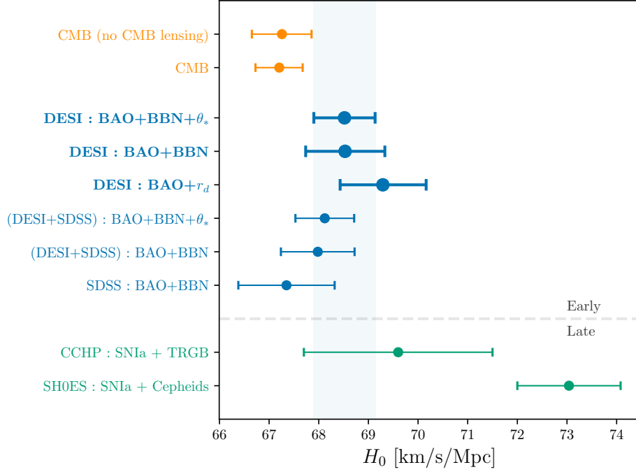
Figure 9. 68% credible-interval constraints on the Hubble constant, assuming the flat \Lambda CDM model. The blue, bold whiskers show DESI BAO measurements in combination with an external BBN prior on \Omega_b h^2 and measurement of the acoustic angular scale \theta_* , the BBN prior alone, or with the CMB measurement of the sound horizon, r_d^{Planck} . The thin blue whiskers show the corresponding results from SDSS BAO and the combination of DESI+SDSS BAO results, as labelled. The orange whiskers show the results from CMB anisotropy measurements from Planck and ACT, while the green whiskers show measurements of H_0 from the distance ladder with either Cepheids or TRGB.
