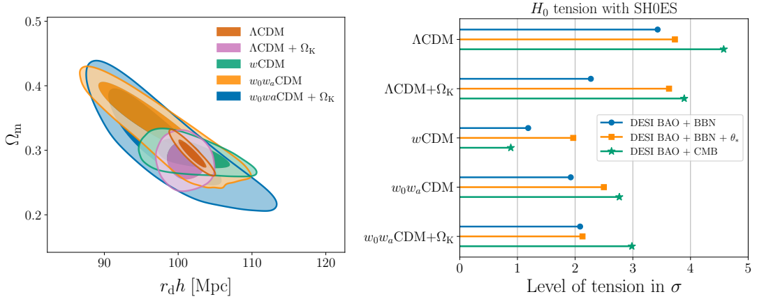
Figure 10. Left panel: The 68% and 95% credible-interval contours for \Omega_m and r_d h obtained from fitting DESI DR1 BAO data in the base flat \Lambda CDM model and in four extension models which modify the background geometry or late-time expansion history. Right panel: A summary of the tension in the H_0 measurements obtained from the DESI BAO results combined with other data, and the SH0ES result of [225], assuming different cosmological models.
