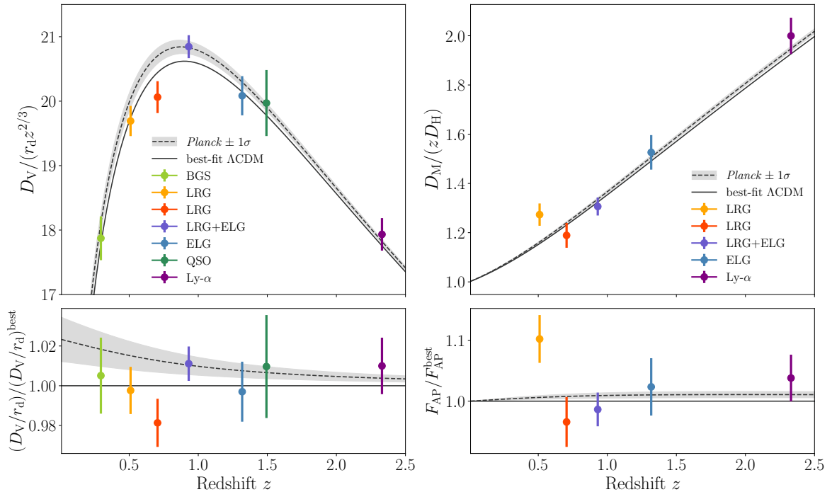
Figure 1. Top row: DESI measurements of the BAO distance scales at different redshifts, parametrized as ( left ) the ratio of the angle-averaged distance D_V \equiv (z D_M^2 D_H)^{1/3} to the sound horizon at the baryon drag epoch, r_d , and ( right ) the ratio of transverse and line-of-sight comoving distances F_{\text{AP}} \equiv D_M/D_H , from all tracers and redshift bins as labeled. For visual clarity and to compress the dynamic range of the plot, an arbitrary scaling of z^{-2/3} has been applied on the left, and z^{-1} on the right. The solid and dashed grey lines show model predictions from, respectively, the flat \Lambda CDM model that best fits this data, and from a \Lambda CDM model with parameters matching the Planck best-fit cosmology. The BGS and QSO data points appear only in the left panel and not the right one because the signal-to-noise ratio of the data is not yet sufficient to measure both parameters for these tracers. Bottom row: The same data points and models as in the top row, but now shown as the ratio relative to the predictions for the best-fit flat \Lambda CDM model.
