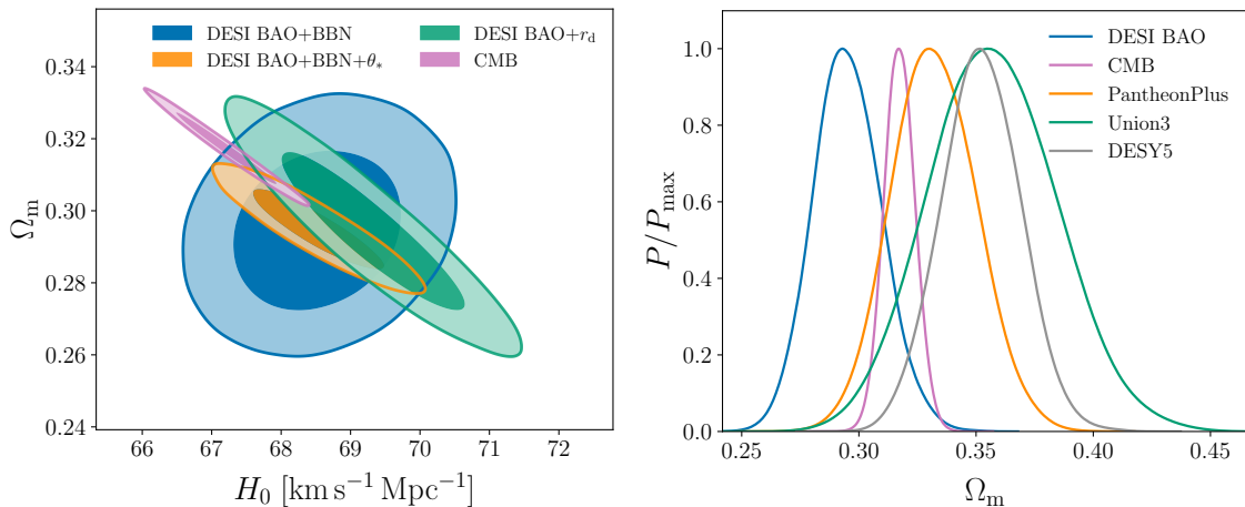
Figure 3. Left panel: marginalized posterior constraints on matter density \Omega_m and the Hubble constant H_0 , obtained from combining DESI BAO data with external data used to calibrate the sound horizon r_d , in a flat \Lambda CDM cosmological model. The combinations shown use a prior on \omega_b determined from BBN (blue), the combination of a BBN \omega_b prior and measurement of the acoustic angular scale \theta_* (orange), and r_d directly calibrated from CMB results from Planck (green). The pink contour shows the corresponding constraints from the combination of CMB and CMB lensing. Right panel: The marginalized 1D posteriors on \Omega_m in flat \Lambda CDM, from DESI BAO, CMB and the three SN datasets, as labelled.
