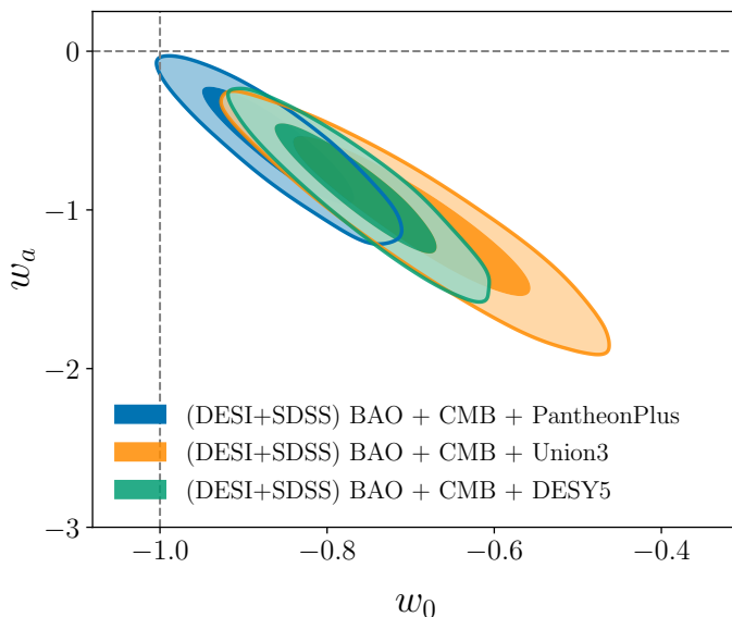
Figure 12. The 68% and 95% marginalized posterior constraints from DESI+SDSS BAO combined with CMB and each of the PantheonPlus, Union3 and DESY5 SN Ia datasets. Compared to cases with DESI DR1 BAO shown in the right panel of Figure 6 all contours are very consistent but the significances of the tensions with \Lambda CDM marginally decrease.
