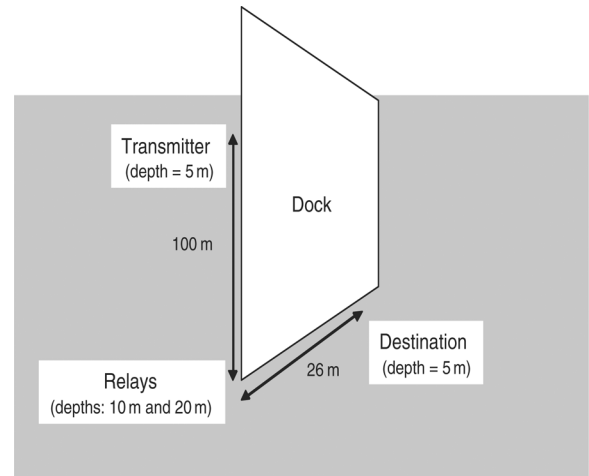
Fig. 8. Experimental setup.
