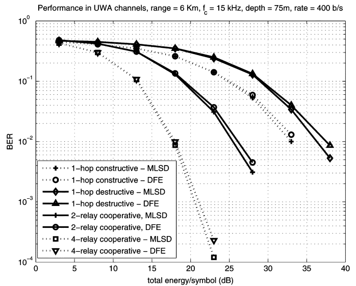
Fig. 4. Two-hop cooperation performance.
