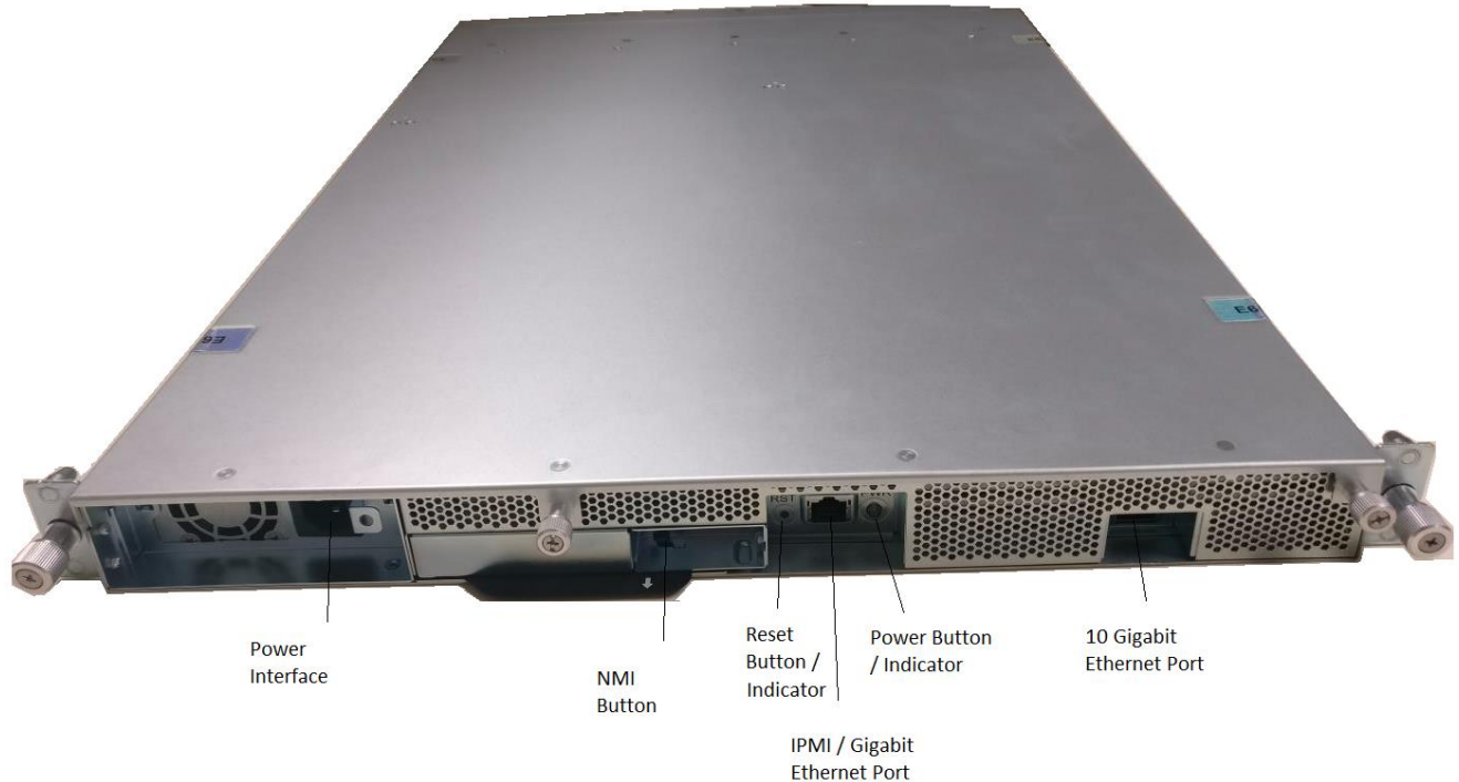
Figure 1 – Cryptographic Module Boundary
