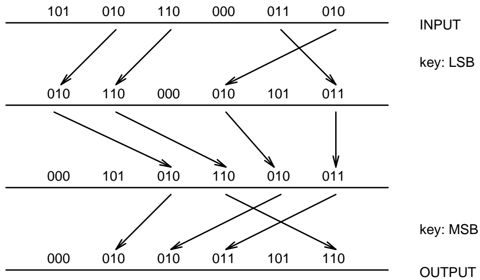
Figure 3.3 Radix Sort: an illustration.
