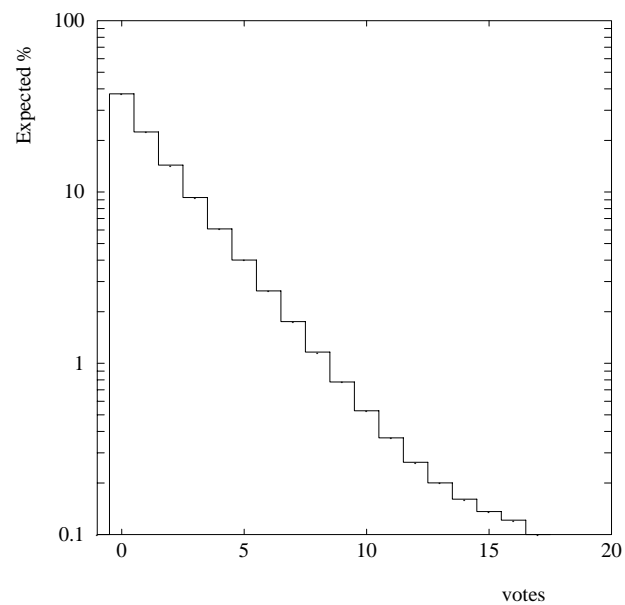
Figure 6.1 Similarity Transforms: the expected percentage of model/basis combinations receiving exactly k votes. Top: the models' feature points are distributed according to a Gaussian of \sigma=1 . Bottom: the models' feature points are distributed uniformly over the unit disc. In both cases, the database contained 512 models, each consisting of 16 points.
