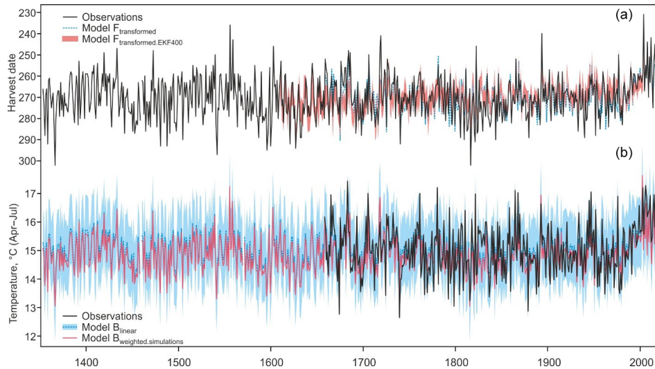
Figure 8. (a) Harvest dates in observations and modelled from observed and reconstructed (EKF400) temperatures. (b) April-to-July mean temperature from observations and reconstructed from models B_{linear} and B_{weighted.simulations} . Blue shading denotes the 95 % prediction interval for B_{linear} .
