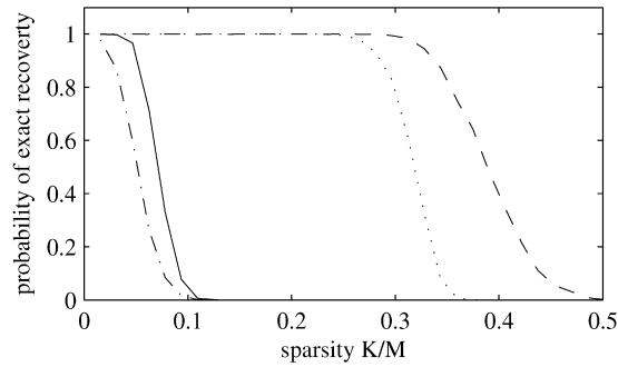
Fig. 1. Comparison in terms of exact support recovery between the Iterative Hard Thresholding algorithm (solid), the CoSaMP algorithm using three conjugate gradient steps (dash-dotted), the CoSaMP algorithm using exact solutions to the inverse problem in each iteration (dotted) and the \ell_1 based method (dashed).
