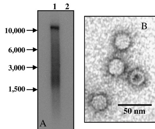
Fig. 1. (A) Northern blot of RNA prepared from purified SINV-3 particles (lane 1) and SINV-3-uninfected fire ant workers (lane 2). Numbers to the left of the blot indicate the size (in nucleotides) of single-stranded RNA standards. (B) Electron micrograph of a negative stain of purified SINV-3 used for the Northern analysis.
