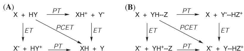
Scheme 1. Square schemes for PCET.
