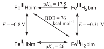
Scheme 3. Thermochemistry of iron–biimidazoline complexes in MeCN ( E vs. \text{Cp}_2\text{Fe}^{+/0} ).
