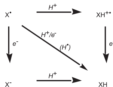
Scheme 2. Square scheme for net H \cdot transfer.
