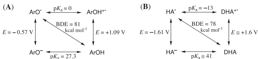
Scheme 4. Thermochemistry of 2,4,6- t\text{Bu}_3\text{C}_6\text{H}_2\text{OH} ( \text{ArOH} ) and dihydroanthracene ( \text{DHA} ) in MeCN ( E vs. \text{Cp}_2\text{Fe}^{+/0} ) [21]; \text{HA}^\cdot and \text{HA}^- refer to the hydroanthracenyl radical and hydroanthracenyl anion, respectively.
