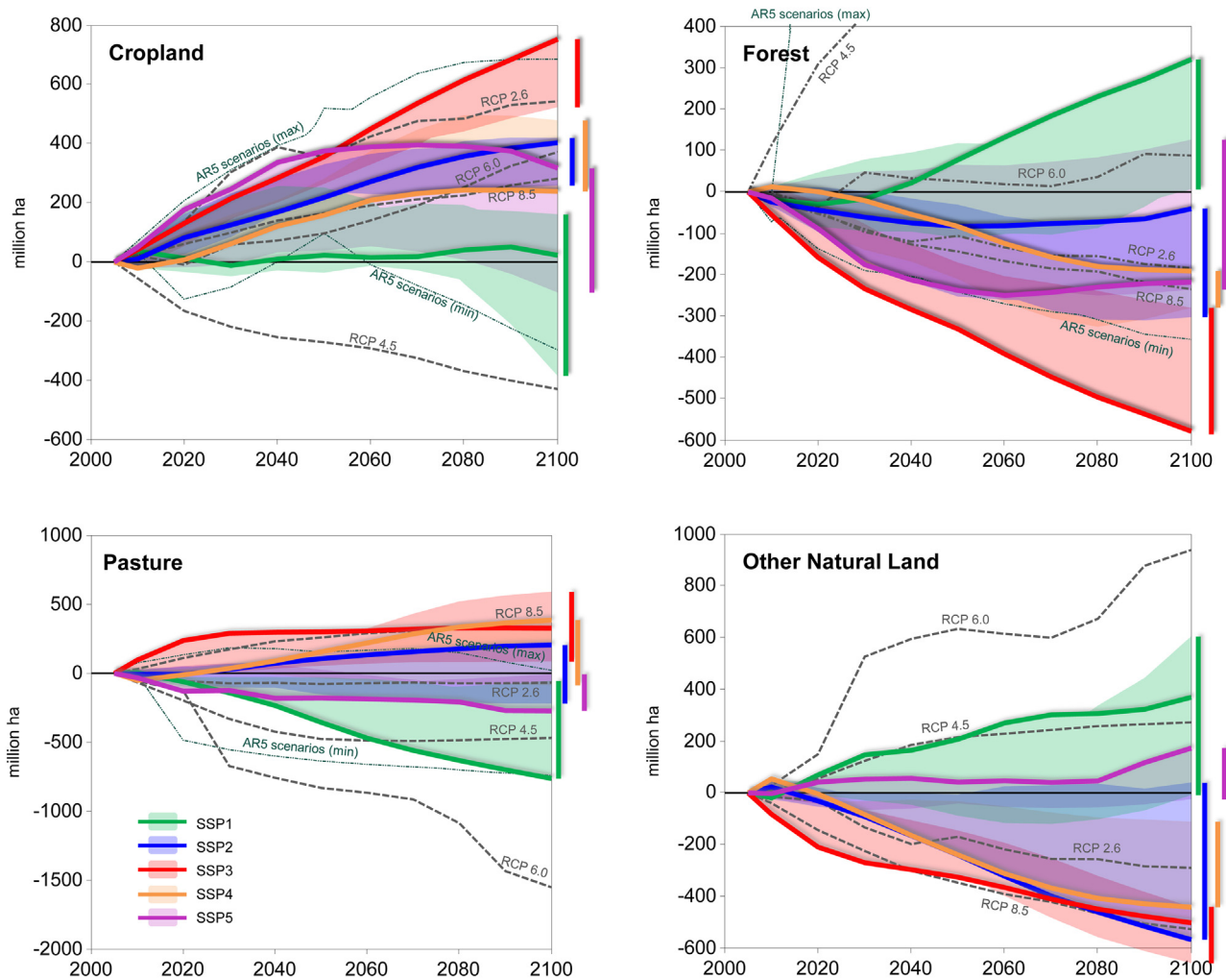
Fig. 4. Changes in cropland, forest, pasture and other natural land for the SSP marker baseline scenarios (thick lines) and ranges of other non-marker scenarios (colored areas). Changes are shown relative to the base year of 2010 = 0. In addition to the SSP baseline scenarios also the development of the RCPs (van Vuuren et al., 2011) and the range of the IPCC AR5 scenarios are shown (Clarke et al., 2014). Note that cropland includes energy crops. Other natural land includes all land-categories beyond forests, pasture, cropland, and build-up areas (the latter category is comparatively small and has not been quantified by all models).
