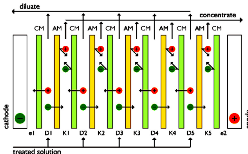
Figure 12 Electrodesalination principles (Chen, 2004). CM – cation-exchange membrane, D – diluate chamber, e1 and e2 – electrode chambers, AM – anion exchange membrane, and K – concentrate chamber.
